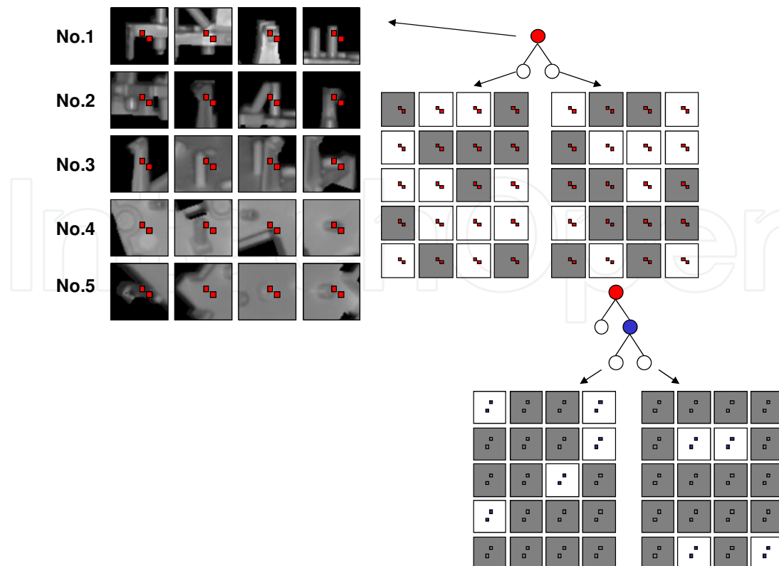
Fig. 3. Patch data partitioning. Based on a comparison of two pixel values, divide a set of patches into two groups with the same content (i.e., left or upper pixel value is larger or not than the other).
