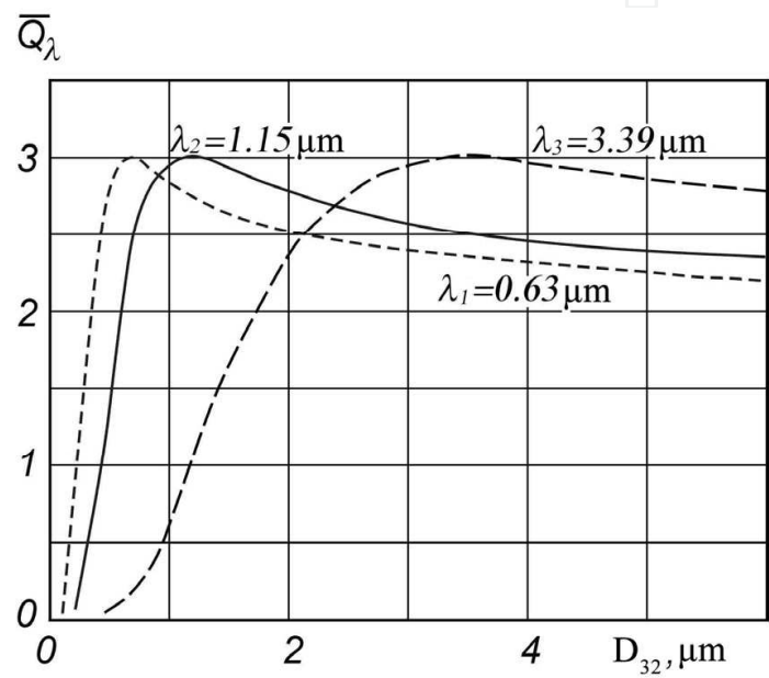
Fig. 1. The averaged attenuation efficiency factors of radiation \bar{Q} plotted against the mean volumetric-surface particle diameter D_{32}
