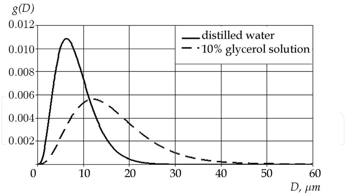
Fig. 12. Mass droplet distribution after spraying (time, 6 s)
