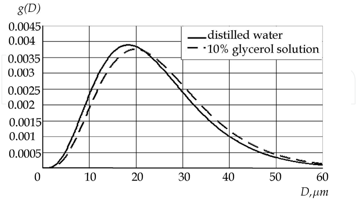
Fig. 11. Mass droplet distribution after spraying (time, 1 s)
