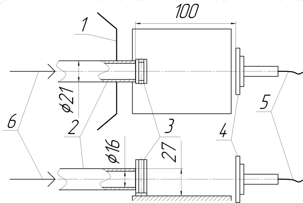
Fig. 3. The cuvette compartment of the measuring complex
