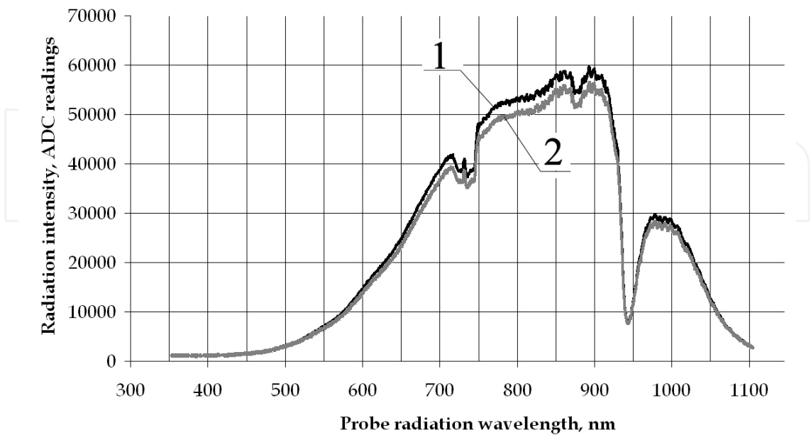
Fig. 4. The optical radiation transmission spectra: 1 – cuvette transmission spectrum with pure distilled water; 2 – cuvette transmission spectrum with \text{Al}_2\text{O}_3 suspension
