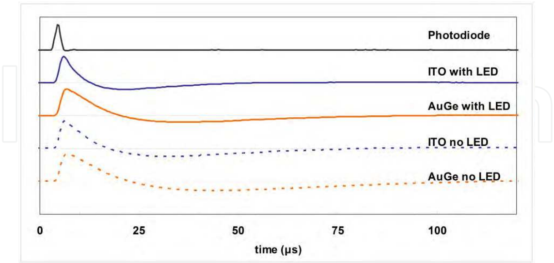
Fig. 2. Plot of GaAs photoconductor response to a 3 \mu s long laser diode pulse for various devices with and without LED background illumination. The response from a silicon photodiode is shown for comparison. The values on the y-axis are normalized (arbitrary units) (Bessette, 2006).
