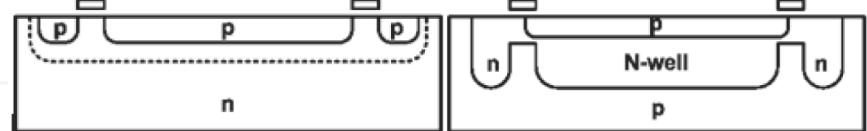
Fig. 5. Double low-doped n-well structure with gates (left) and guard rings and control gate signal (right). Termination techniques (4) and (5) in table 3, respectively.
