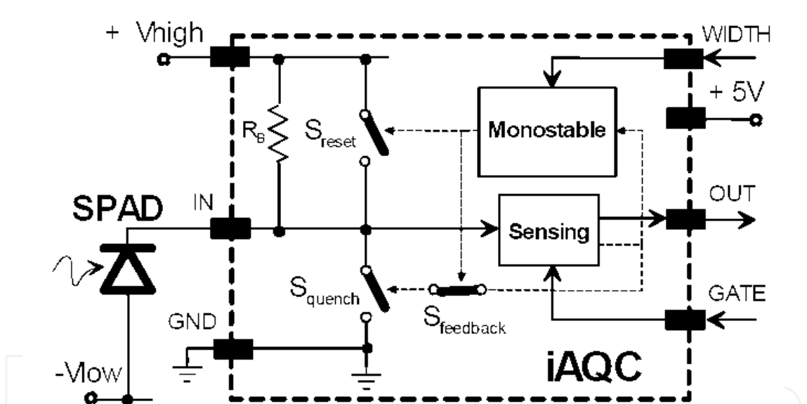
Fig. 19. Integrated active quenching and recharge structure (Zappa et al., 2002).
