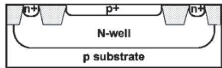
Fig. 6. Structure to avoid PEB based on STI elements. Termination technique (6) in table 3.
