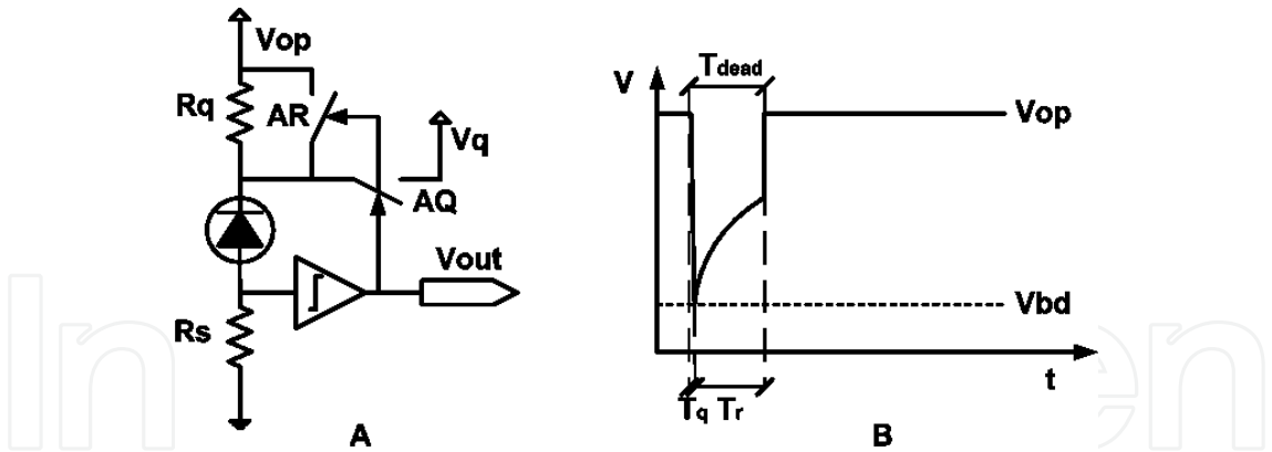
Fig. 18. A) Active quenching by switch AQ and recharge by switch AR. B) Sketch of the timing behaviour.
