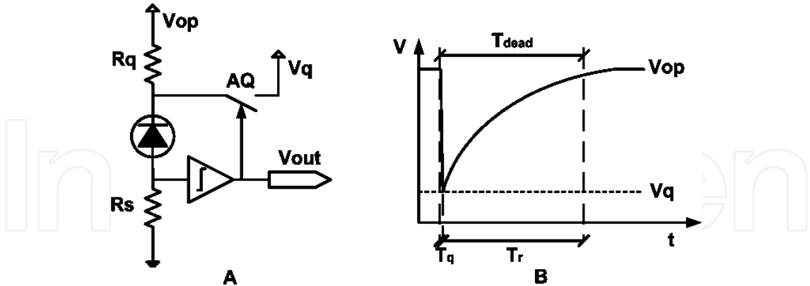
Fig. 17. A) Active quenching with passive recharge. B) Sketch of the timing behaviour.
