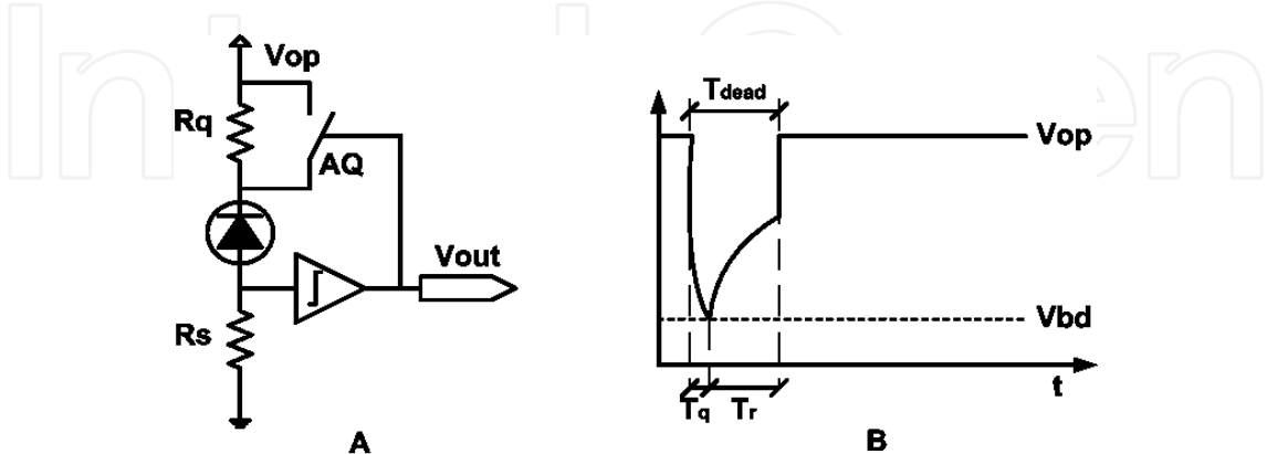
Fig. 16. A) Passive quenching and active recharge by a switch AQ. B) Sketch of the timing behaviour.
