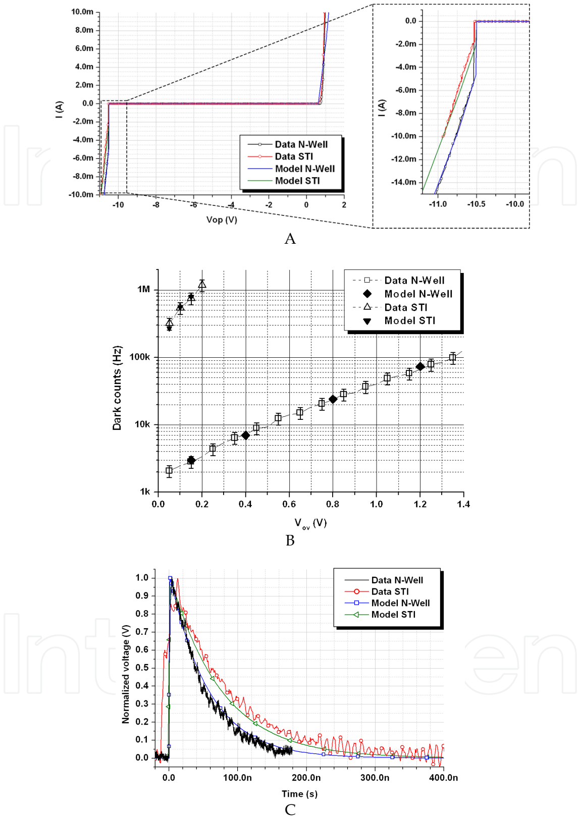
Fig. 13. A) I-V measurements and simulation using the models for an N-well and a STI structures. B) Dark counts measured for the N-well and the STI structures with a 10 kΩ quenching resistance. C) Time response of the two structures and the models represented with a normalized voltage and a quenching resistance of 10 kΩ.
