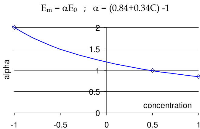
Fig. 14. Alpha as a function of normalized concentration (Kringos et al., 2012)
