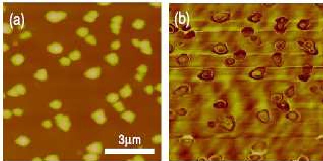
Fig. 8. (a) AFM and (b) MFM images of the sputter-deposited SiMn 20% film after thermal annealing at 600 °C. The AFM scanning was performed in the tapping mode, whereas MFM in the lift mode by means of a Co/Cr coated tip magnetized just before scanning. The measurements were carried out under room conditions (temperature and atmosphere) from a 1.7 μm thick film deposited on crystalline silicon (Ferri et al., 2009a)
