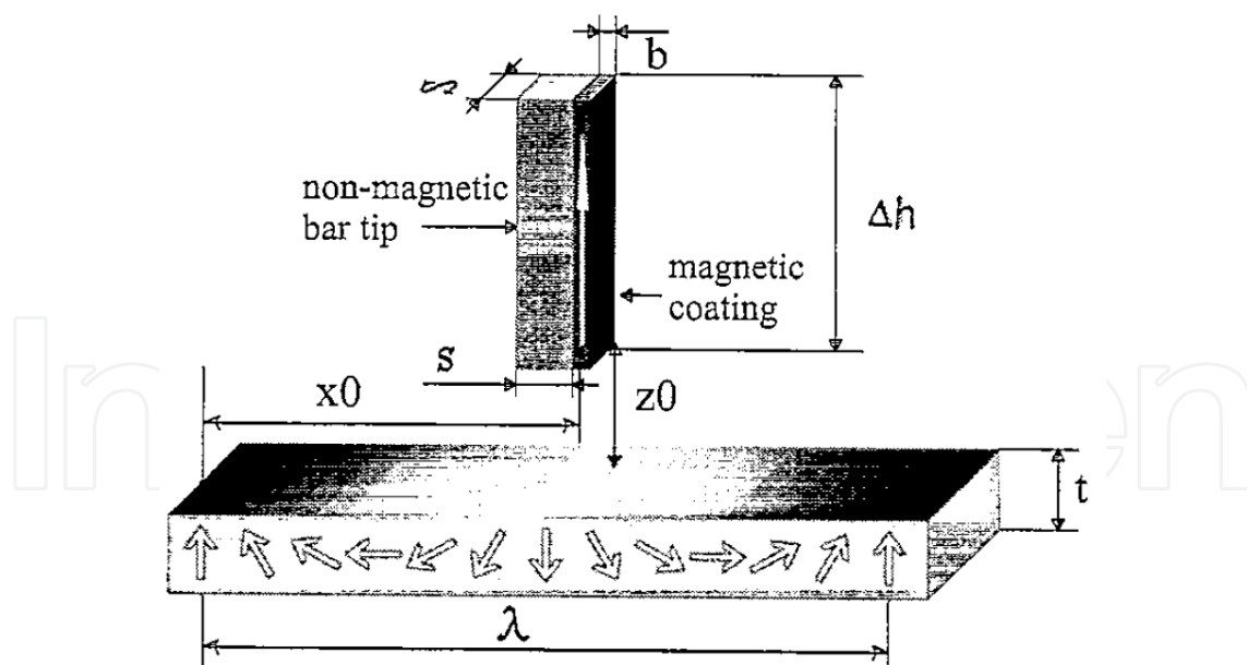
Fig. 4. One-dimensional model for the MFM measurement process (Porthun et al., 1998)
