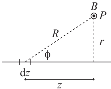
Fig. 3. The Biot-Savart law: magnetic field due to a small segment carrying a current I . The direction of the magnetic field is out of the page.
