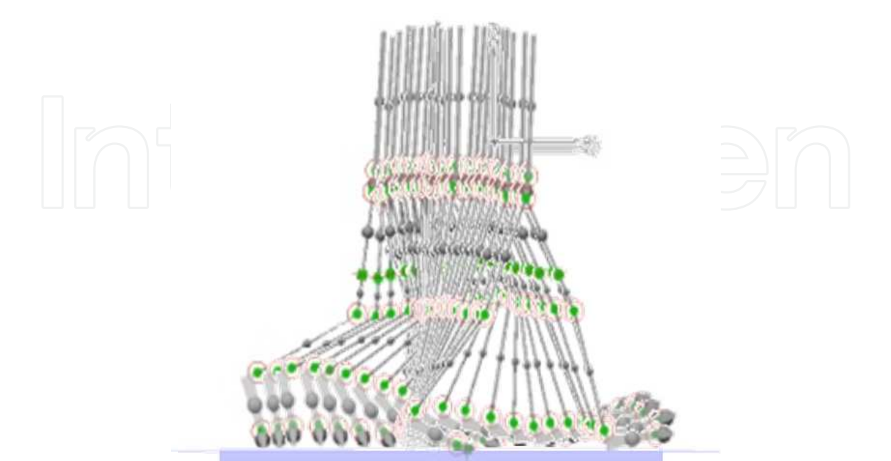
Fig. 4. The sequences of simulation during swing phase.
