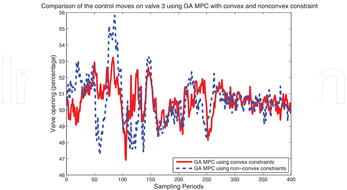
Fig. 11. Comparison of the calculated control moves for control valve 3 (convex vs. non-convex GA-MPC)
