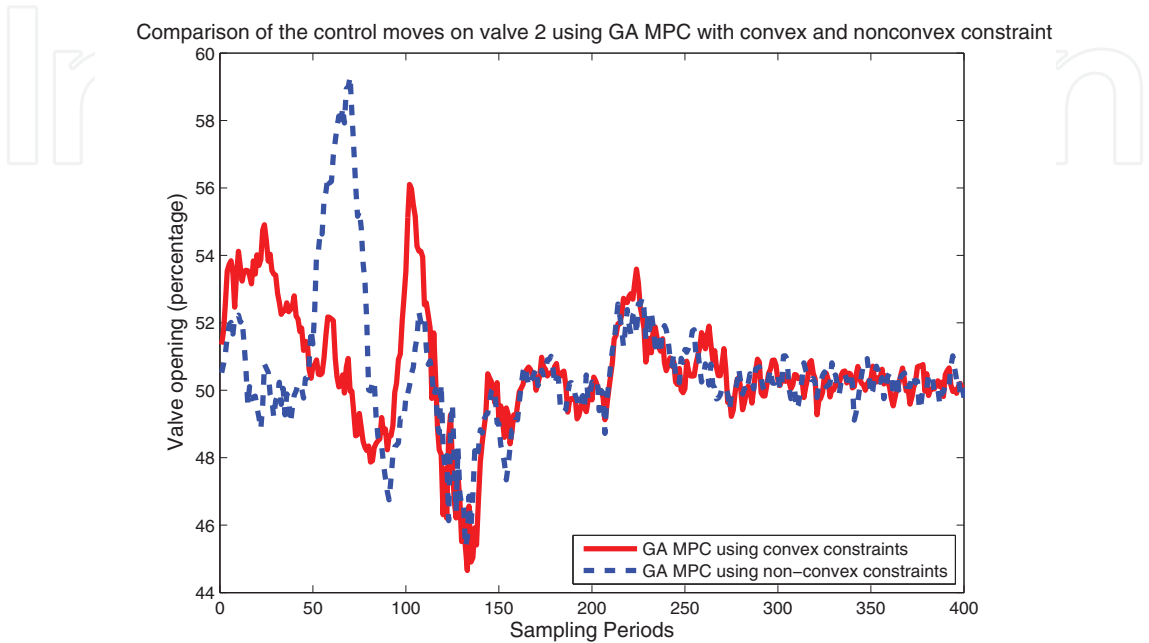
Fig. 10. Comparison of the calculated control moves for control valve 2 (convex vs. non-convex GA-MPC)
