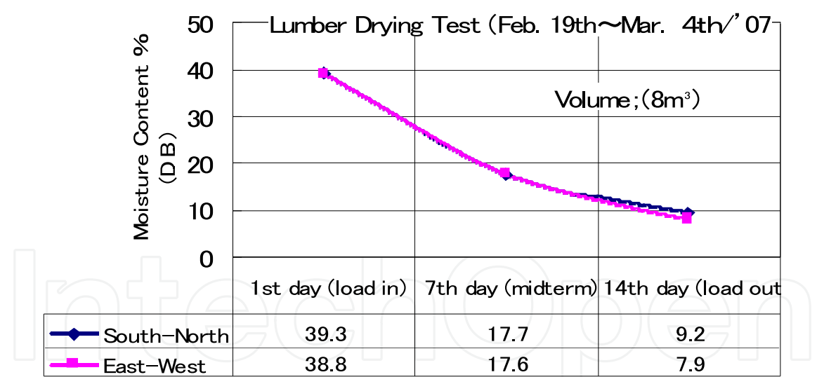
Fig. 15. Comparison of Drying Speed between South-North model & East-West model
