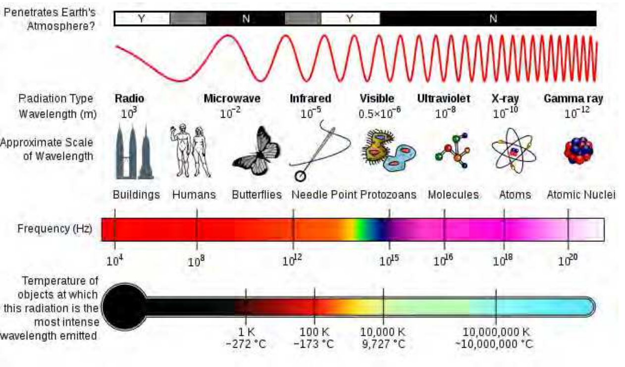
Fig. 1.2. Spectral ranges of electromagnetic radiation
