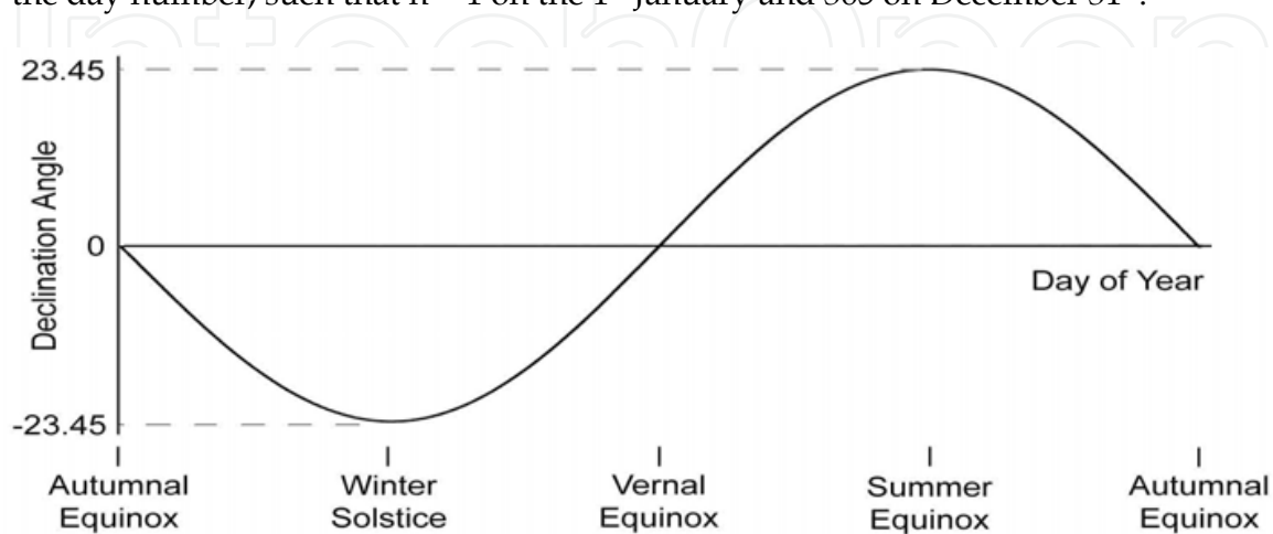
Fig. 1.6. The variation in the declination angle throughout the year.
