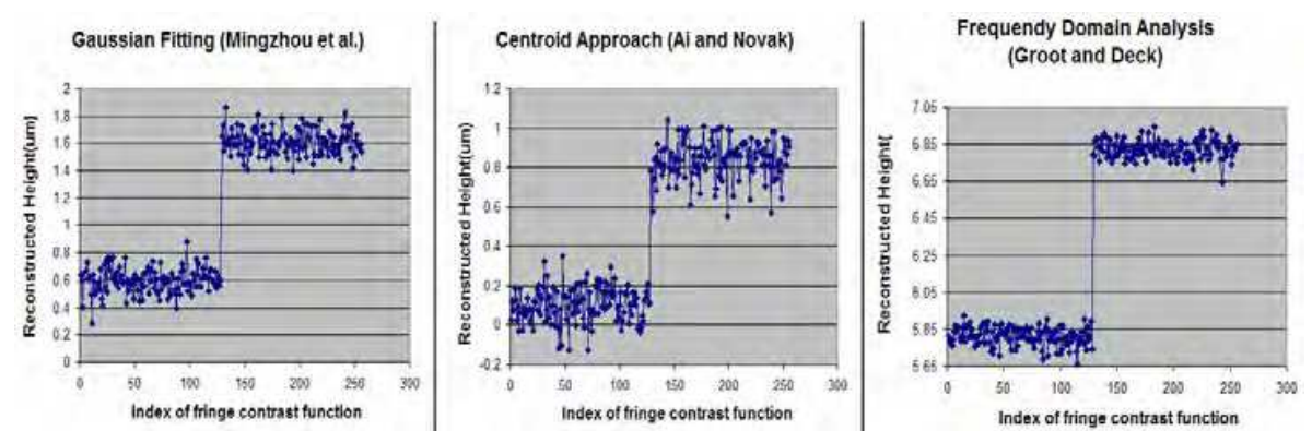
Fig. 9. For phosphor-based LED set, 1um step height reconstructed using (a) Gaussian Fitting by Mingzhou et al. (b) Centroid approach by Ai and Novak (c) Frequency domain analysis by Groot and Deck
