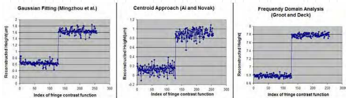
Fig. 10. For light source of Gaussian spectrum, 1um step height reconstructed using (a) Gaussian Fitting by Mingzhou et al. (b) Centroid approach by Ai and Novak (c) Frequency domain analysis by Groot and Deck
