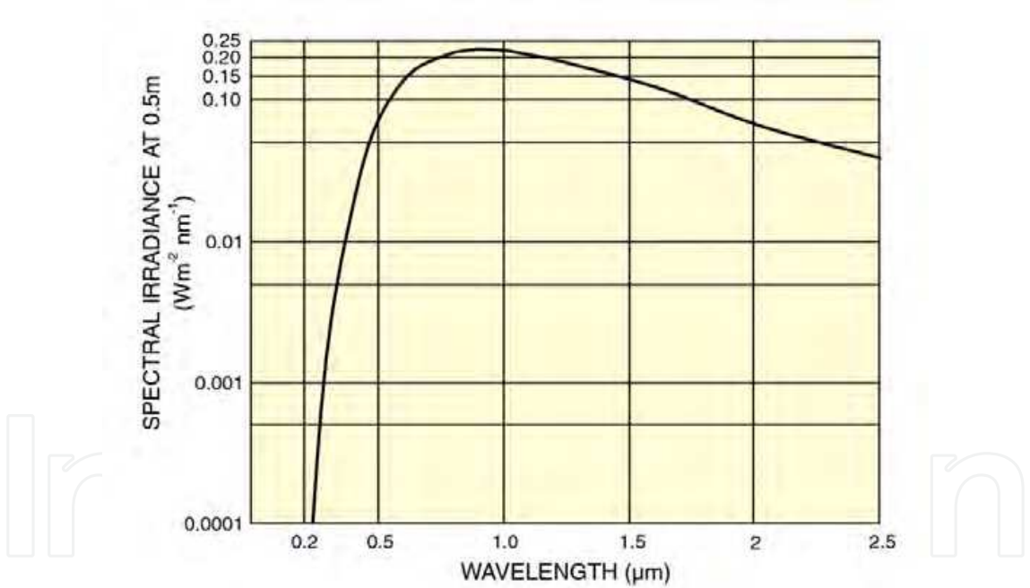
Fig. 4. Spectral irradiance at 0.5 m from the 6315 1000W QTH Lamp3 (by NewPort).
