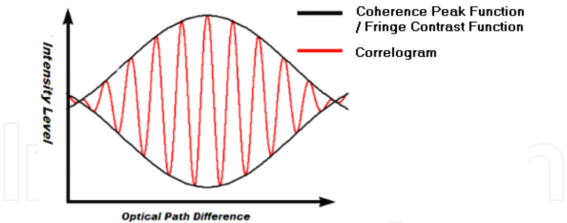
Fig. 3. Example of correlogram and corresponding fringe contrast function (also known as coherence peak function) in vertical scanning interferometry.
