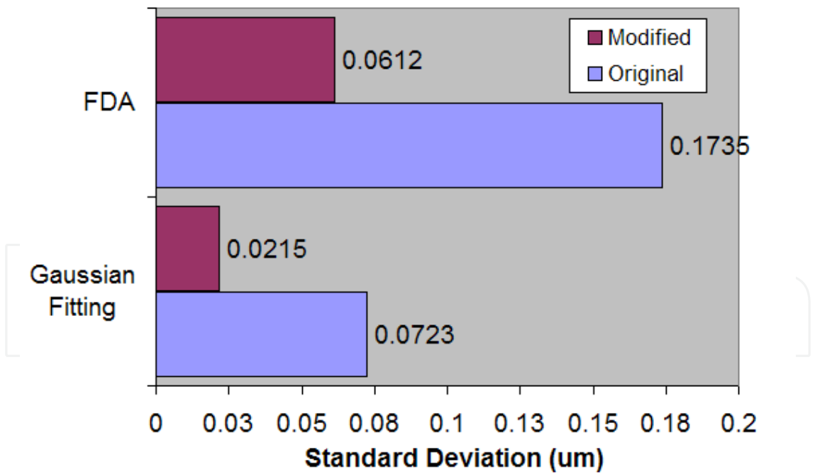
Fig. 15. Simulation verification on the proposed modification: Comparing standard deviation of measuring perfectly flat surface reproduced by proposed modification and original.
