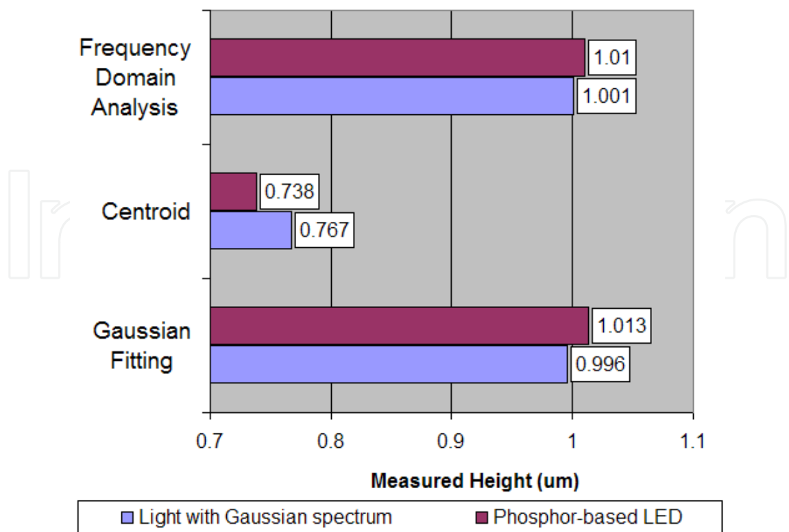
Fig. 11. Comparing measurement accuracy of different algorithms between different light sources, ideal value is 1um.
