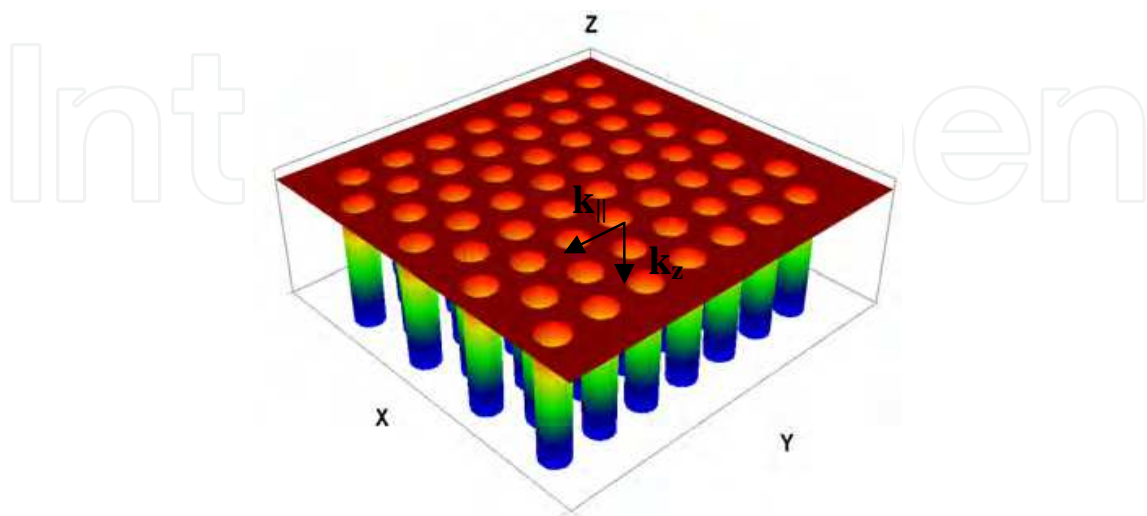
Fig. 7. Modes propagating parallel to the plane of periodicity xy ( k_z=0 ), can be classified in transverse electric (TE) and transverse magnetic (TM) in two dimensional photonic crystals
