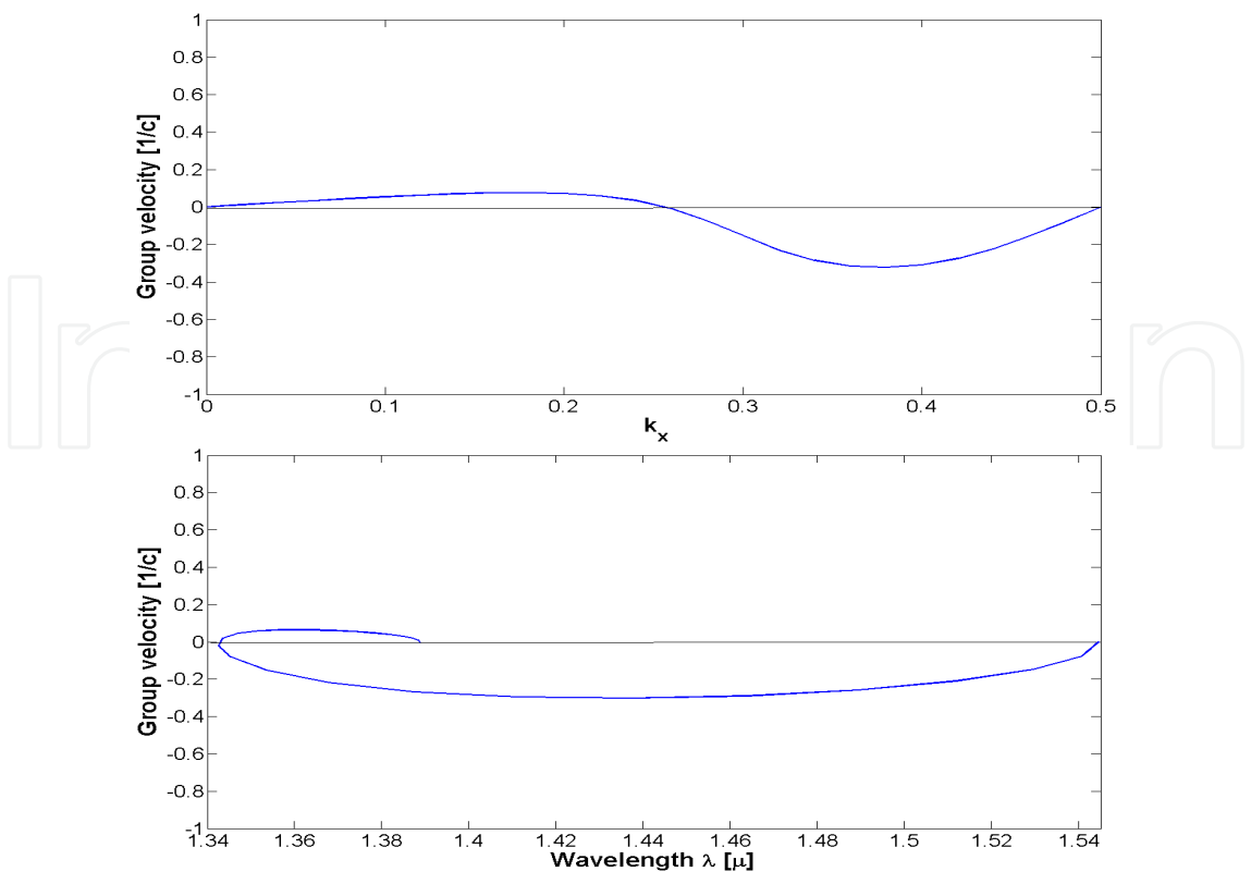
Fig. 11. Group velocity of light pulses coupled to the defect mode confined within the waveguide as a function of wave vector k_x (top) and as a function of wavelength (bottom)
