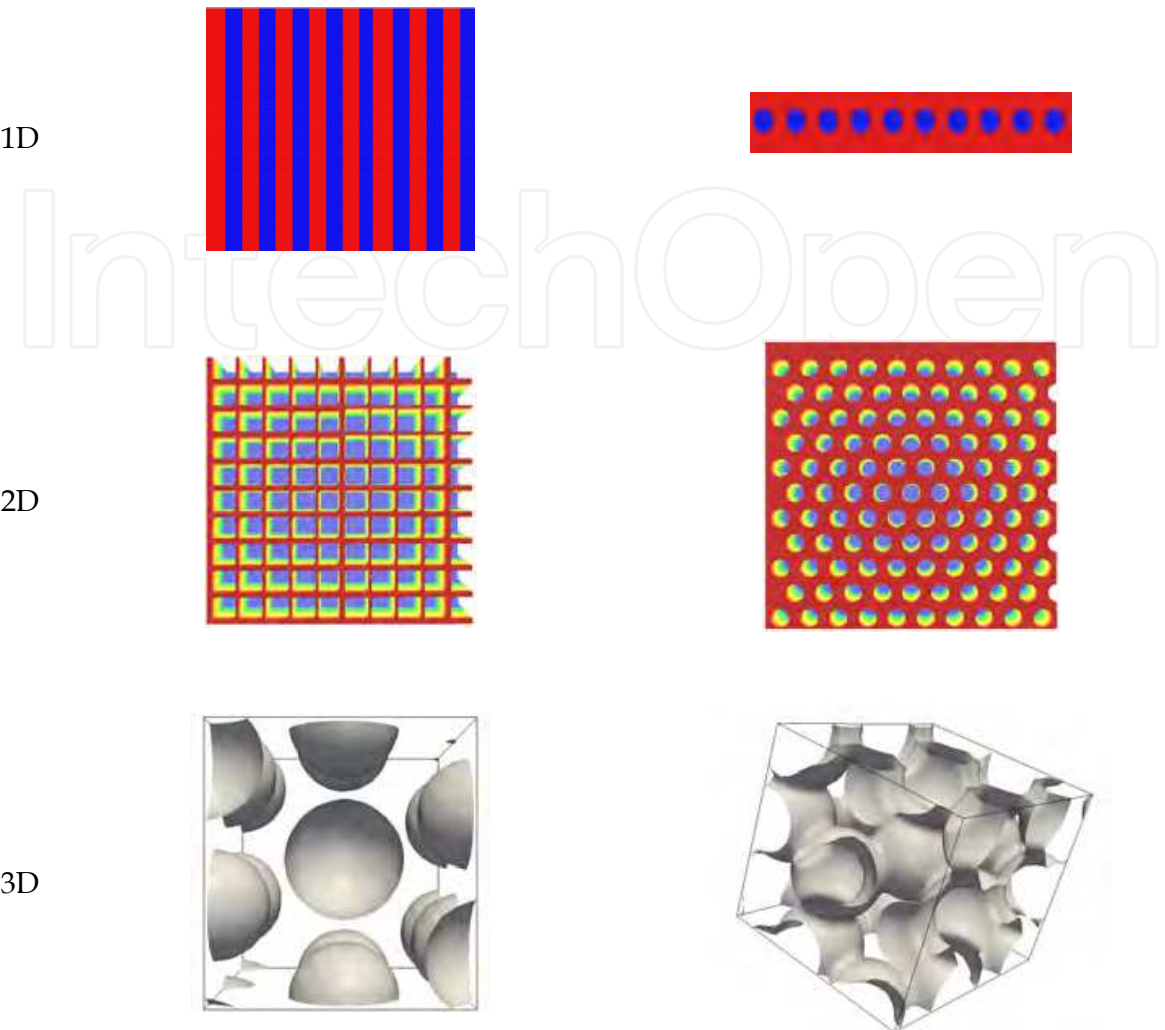
Fig. 6. Examples of one-, two- and three-dimensional photonic crystals.
