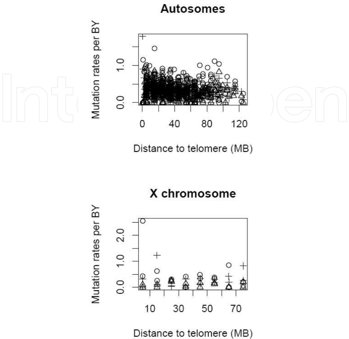
Fig. 3. A scatter plot of the mutation rates on TpG sites versus the distances to telomeres. The open squares (□) show the CpG to TpG mutation rates. The open circles (○) show the TpG to CpG mutation rates. The open triangles (Δ) show the rates of non-CpG transition. The crosses (+) show the rates of transition.
