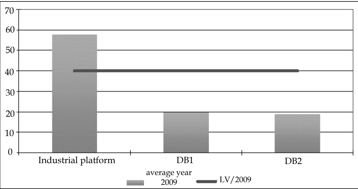
Fig. 11. Average annual concentrations of the PM 10 indicator, measured gravimetrically ( \mu\text{g}/\text{m}^3 ).
