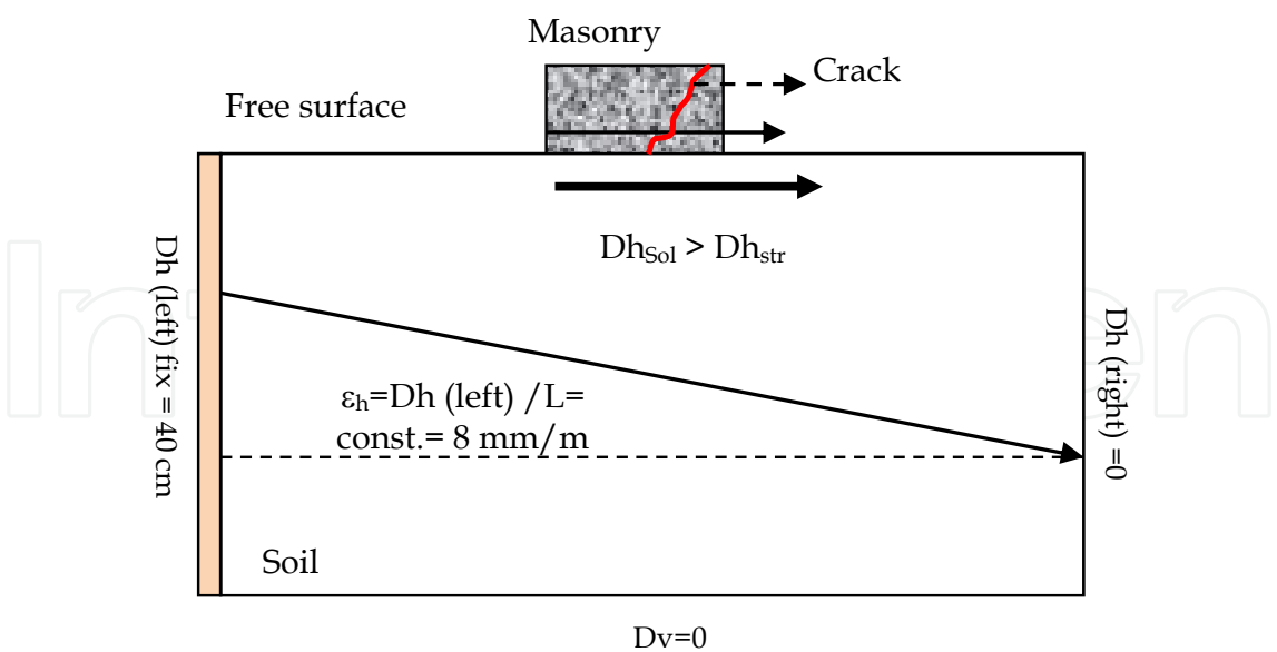
Fig. 27. Analyze of soil structure interaction due to the ground movement.
