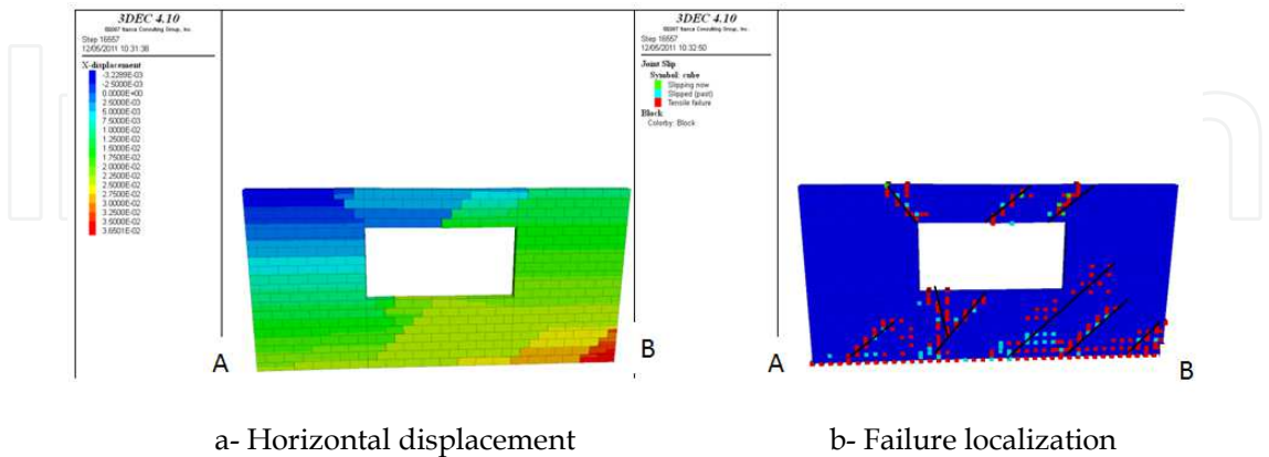
Fig. 24. Behavior of masonry wall under the effect of ground subsidence due to the underground excavation – results obtained by 3DEC numerical model.
