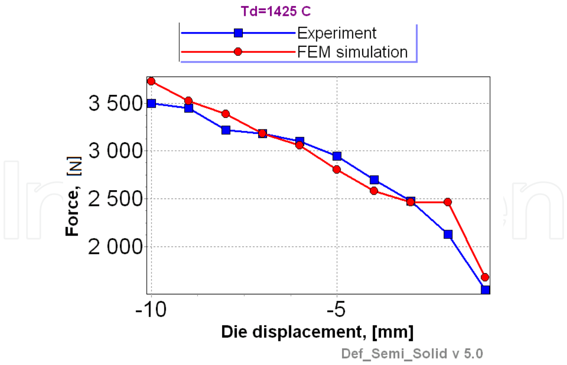
Fig. 17. Comparison between measured and predicted loads at temperature 1425°C.
