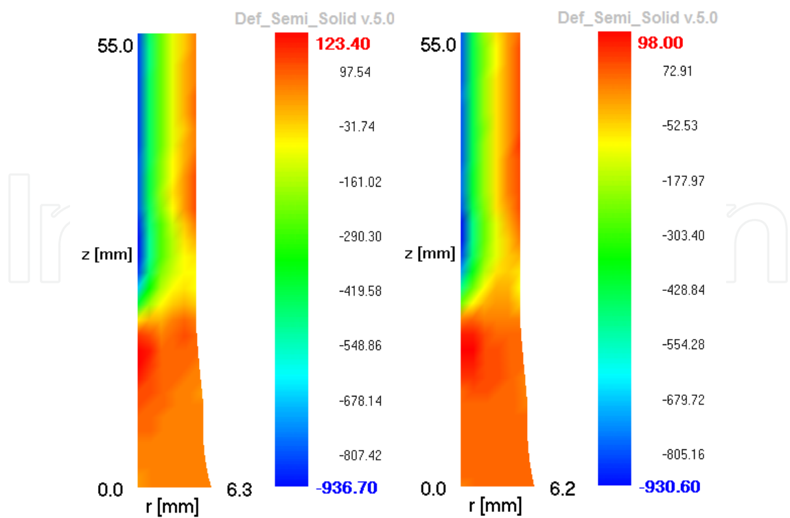
Fig. 21. Example results of computer simulation of deformation at 1350°C (left) and 1425°C (right): final mean stress distribution in the cross-section of the sample.
