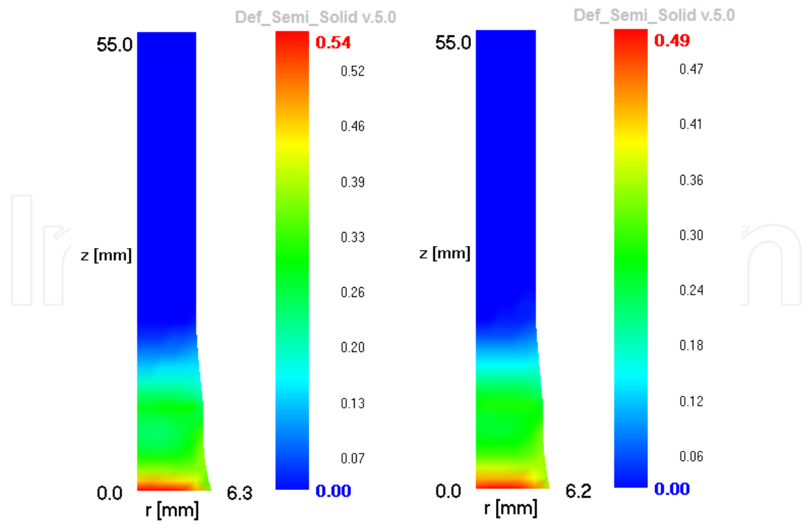
Fig. 20. Example results of computer simulation of deformation at 1350°C (left) and 1425°C (right): final strain distribution in the cross-section of the sample.
