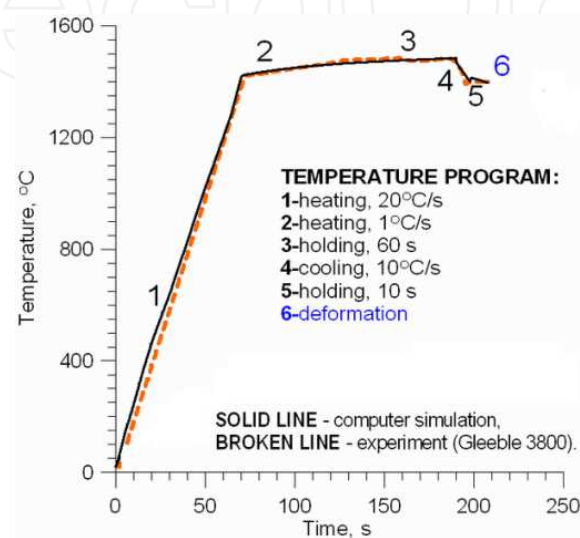
Fig. 10. Comparison between the experimental and theoretical time-temperature curves during initial heating and final compression at 1400°C.
