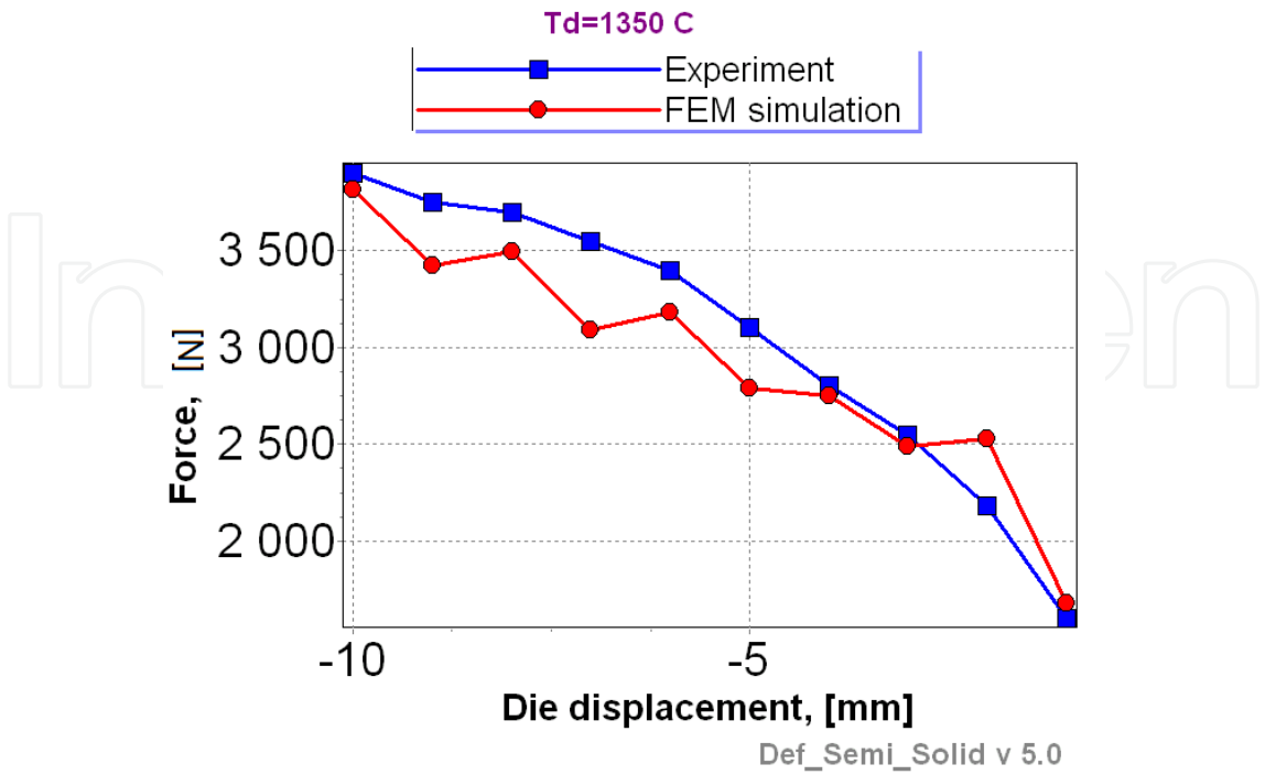
Fig. 15. Comparison between measured and predicted loads at temperature 1350°C.
