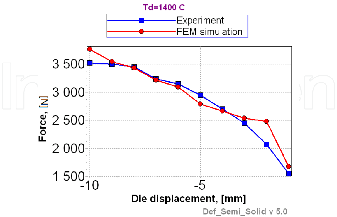
Fig. 16. Comparison between measured and predicted loads at temperature 1400°C.
