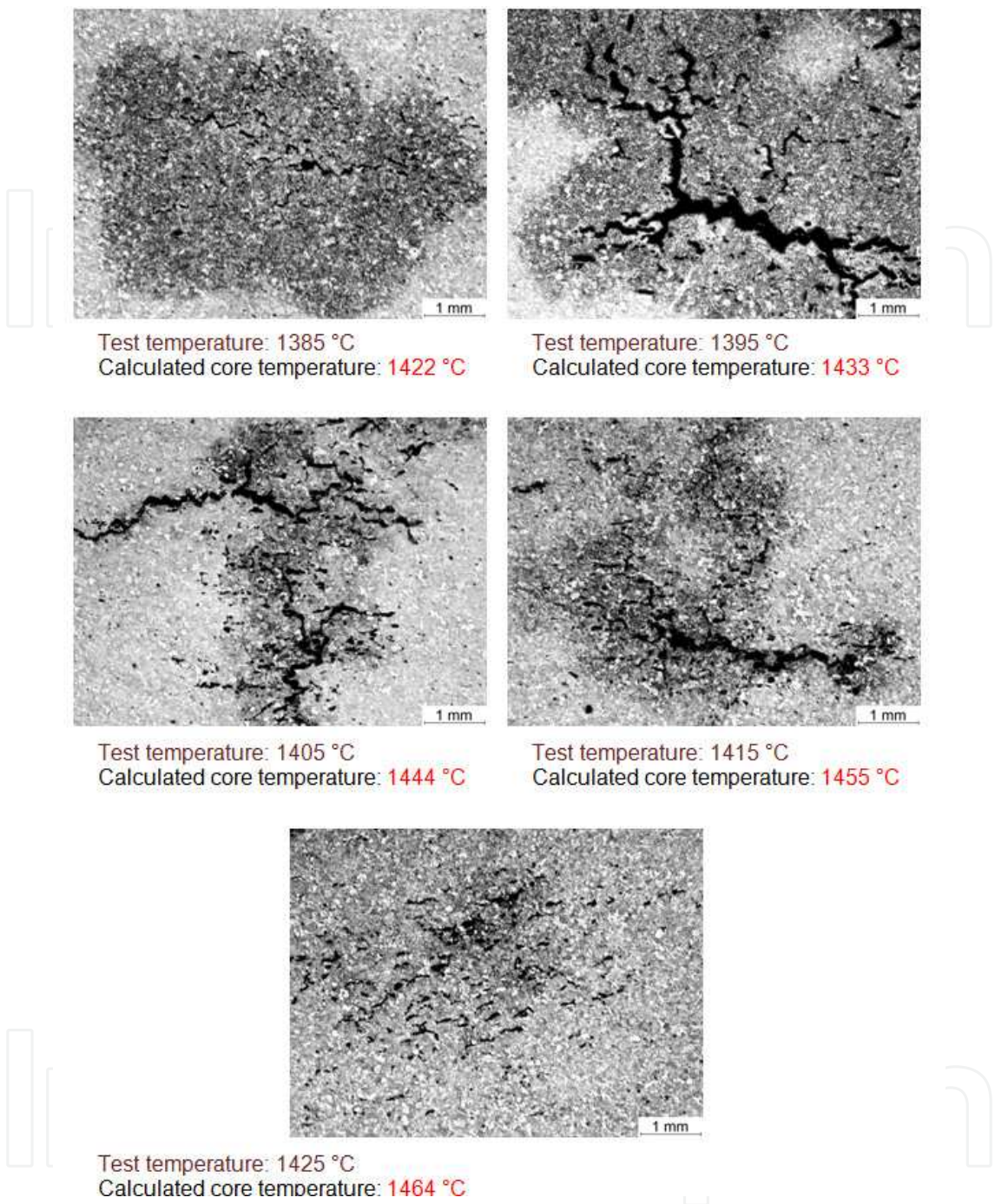
Fig. 14. Macrostructure of the middle of the sample right before deformation. Variant with hot handle. Magnification: 10x.
