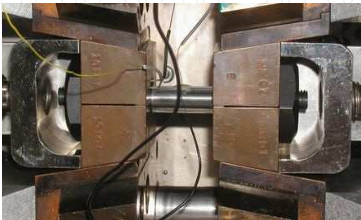
Fig. 4. The standard Gleeble® equipment allowing deformation is semi-solid state.
