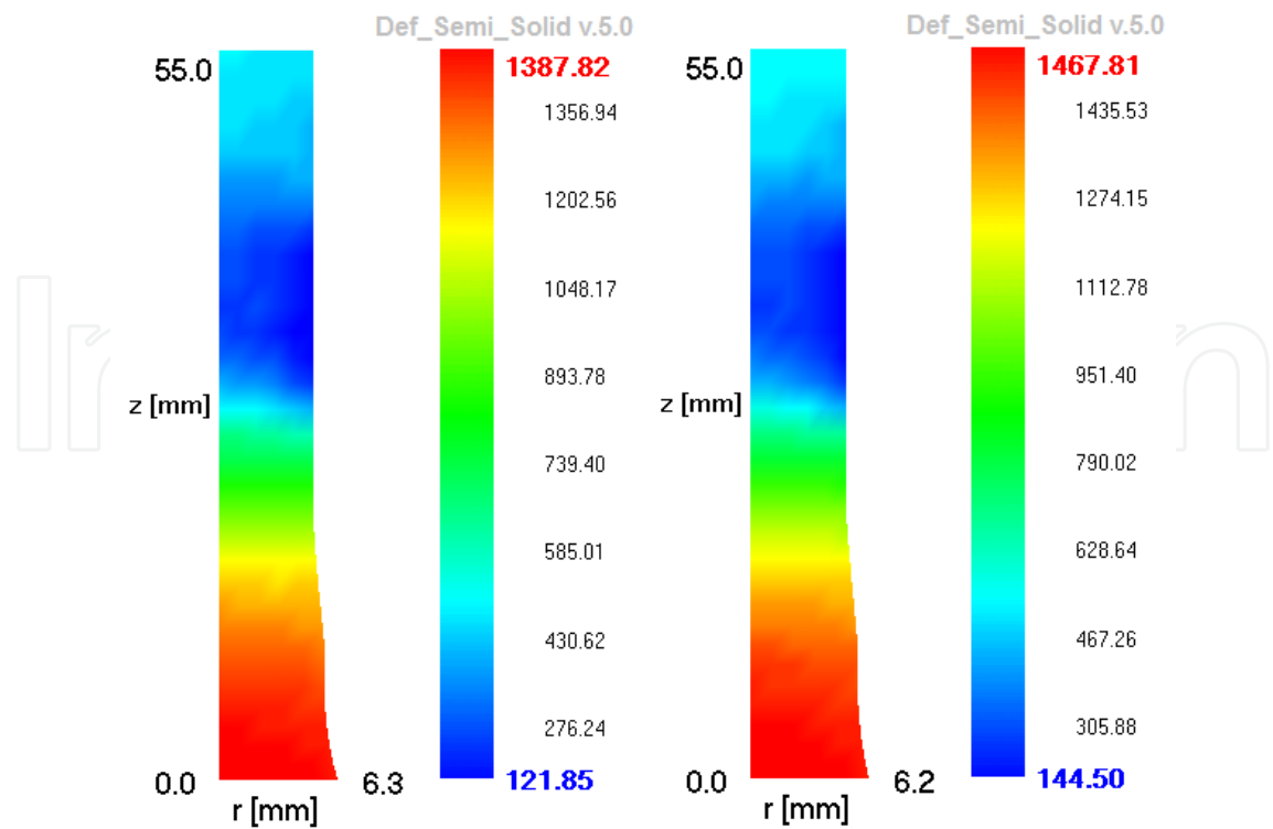
Fig. 19. Example results of computer simulation of deformation at 1350°C (left) and 1425°C (right): final temperature distribution in the cross-section of the sample.
