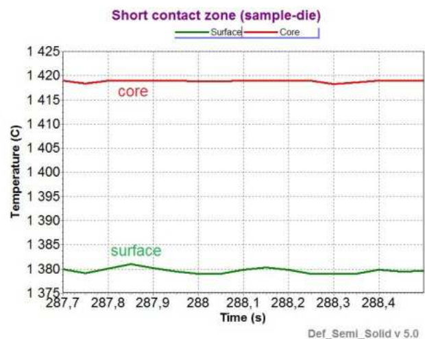
Fig. 11. The temperature change versus time for hot handle (final stage of physical simulation right before deformation at 1380 °C ).
