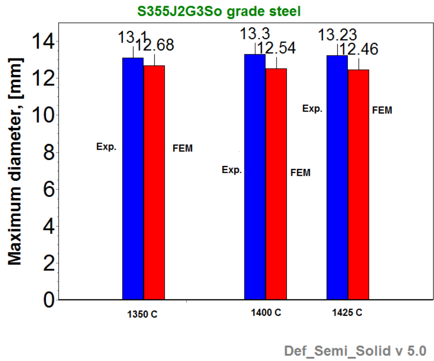
Fig. 23. The comparison of the measured and calculated maximal diameters of the sample – experiments between 1350°C and 1425°C.
