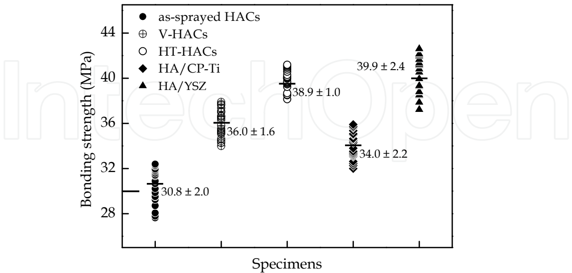
Fig. 8. Results of measuring bonding strength with the average value \pm S.D. and the data fluctuation of as-sprayed HACs, V-HACs, HT-HACs, HA/CP-Ti and HA/YSZ composite coatings (S.D. means the standard deviation).
