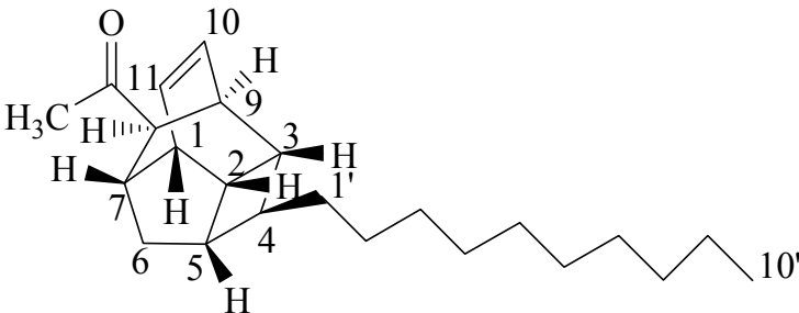
38: Beilcyclone
