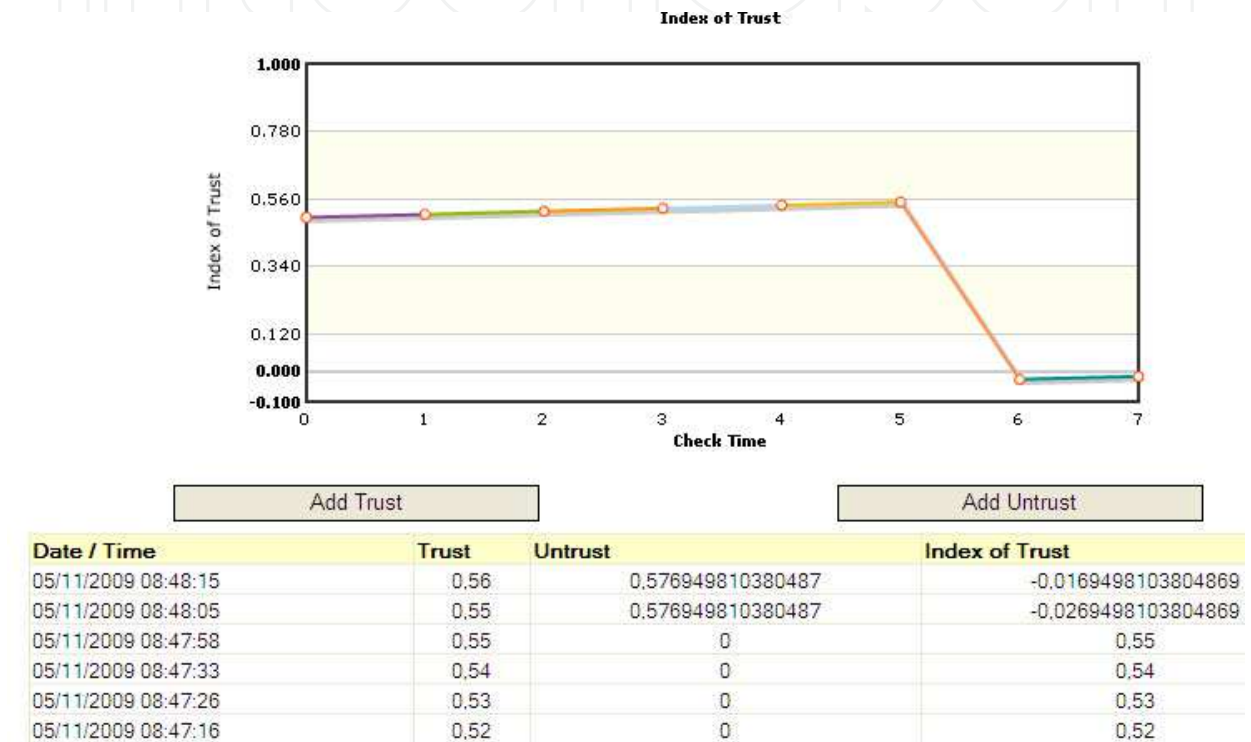
Fig. 6. Trust variation.
