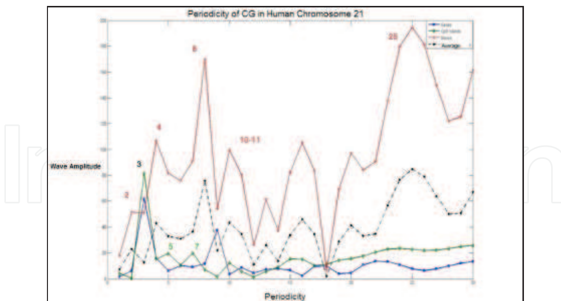
Fig. 2. Fourier analysis (Periodicity Vs Average Wave Amplitude) of global periodicities of CG dinucleotides in 19 Genes (blue line), non-coding near them (red line) and all CpG Islands (green line) in chromosome 21. The average of the 3 region levels is shown as a dotted line.
