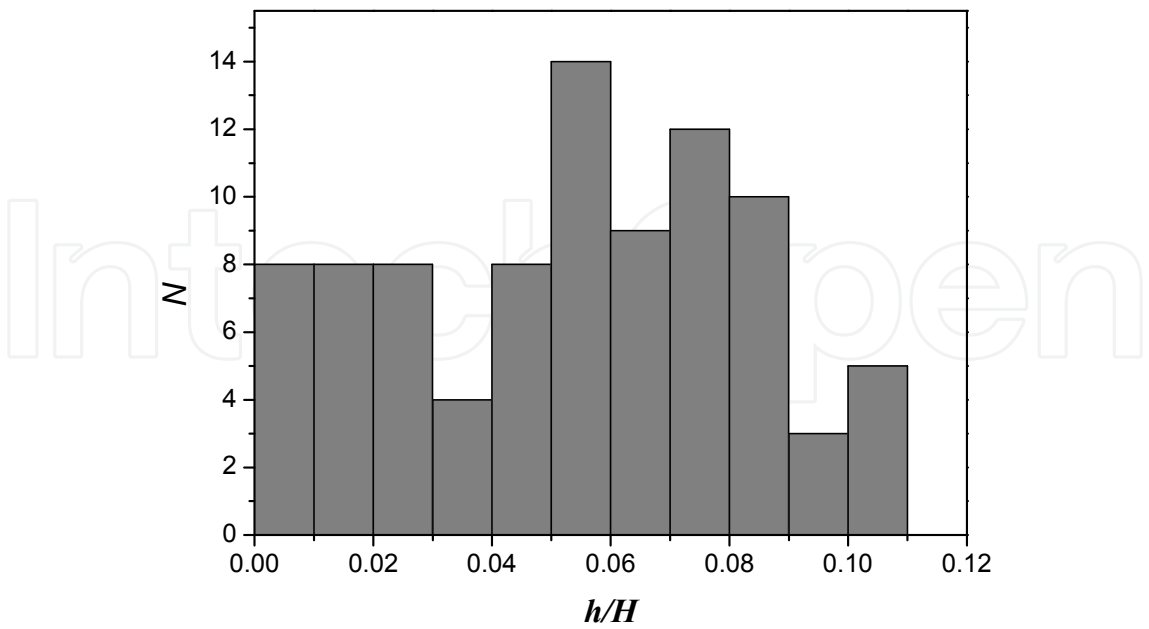
Fig. 12. Distribution of defects over their coordinate h/H near the ingot base: N is the number of defects; h is the distance from a defect to the ingot base; H is the ingot height.
