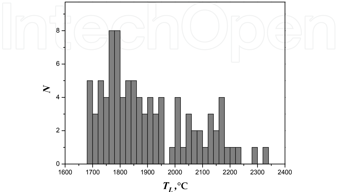
Fig. 5. Distribution of defects over the liquidus temperature of the defect material: N is the number of defects; T_L is the calculated liquidus temperature of the defect material.
