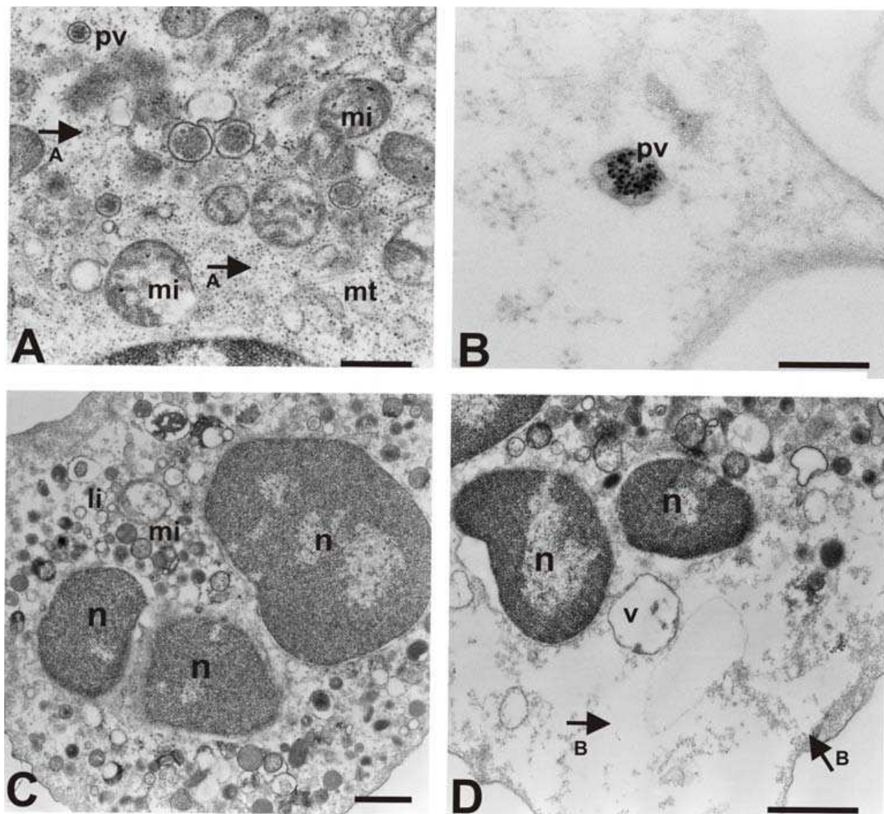
Fig. 3. (A, B) Transmission electronic microscopy of CD133 + stem cells. (C, D) Transmission electronic microscopy of CD133 - stem cells (control). n = nucleus, mi = mitochondria, mt = microtubules, arrow A = electron-dense granules or magnetic nanoparticles, arrow B = absence of the electron-dense granules or magnetic nanoparticles, pv = pinocytotic vesicles, li = lipids, v = vacuoles. Scale: A) 1 \mu m; B) 0,5 \mu m; C) 0,25 \mu m; D) 0,25 \mu m.
