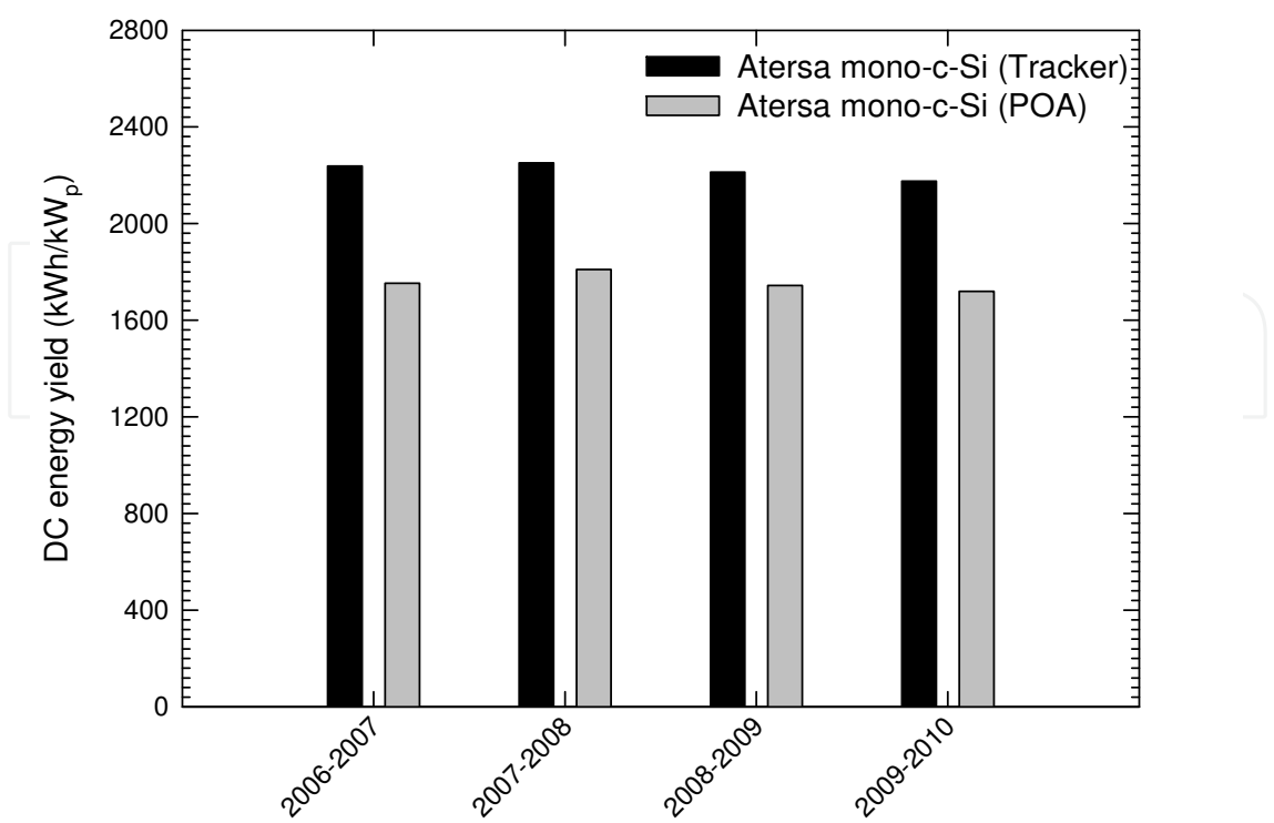
Fig. 1. Comparison of the annual dc energy yield of the tracker and fixed-plane Atersa mono-c-Si systems over the period June 2006 - June 2010.
