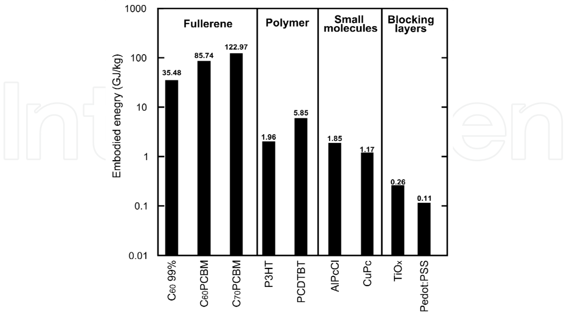
Fig. 10. Cumulative energy demand (CED) for various materials commonly used in organic photovoltaics.
