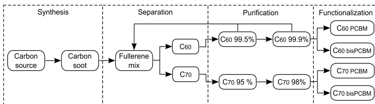
Fig. 5. Overview of the process flow for producing modified fullerene compounds for use as functional materials in organic solar cells (Ancil et al. 2011).
