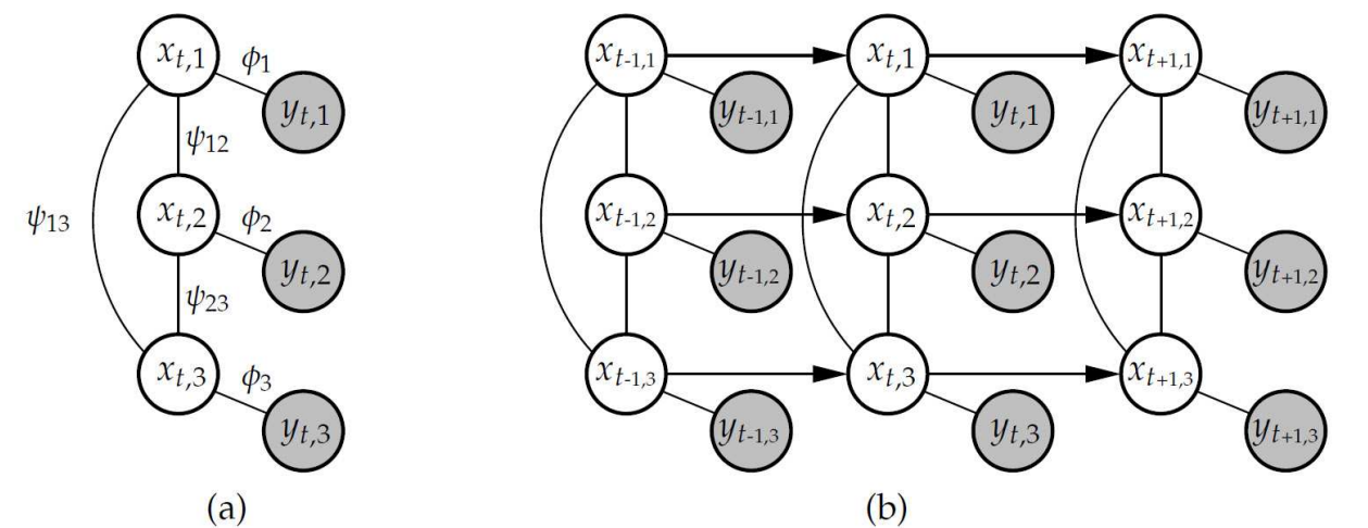
Fig. 2. The graphical model represents the dependence through pairwise potentials (\psi_{12}, \psi_{13}, \psi_{23}) between hidden nodes (x_1, x_2, x_3) , and likelihood functions (\phi_1, \phi_2, \phi_3) between hidden and observable nodes (y_1, y_2, y_3) (a). By introducing temporal potentials between successive nodes (b), the graphical model becomes dynamic and allows for tracking ICP peaks in real time (reproduced from permission from [24]).
