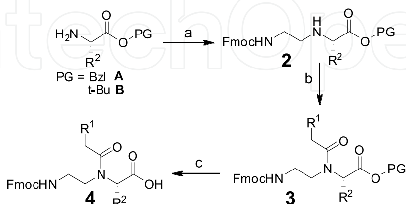
Fig. 5. Synthesis scheme of \alpha -AApeptide building block. a) Fmoc-amino ethyl aldehyde, NaBH_3CN , overnight. b) R_1CH_2COOH , DhBtOH/DIC , overnight. c) Pd/C, H_2 for A ; 50% TFA/CH_2Cl_2 for B . Figure is adapted from (Hu et al. 2011).
