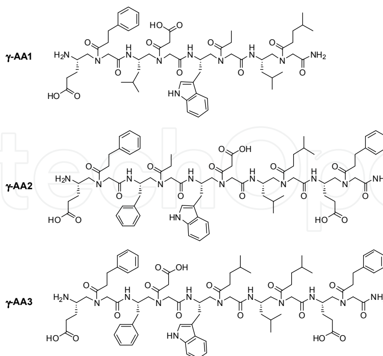
Fig. 3. \gamma -AApeptide sequences designed for p53/MDM2 disruption. Figure is adapted from (Niu et al. 2011).
