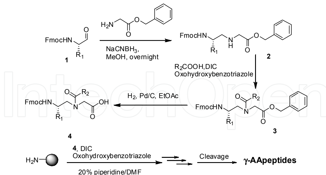
Fig. 6. Synthesis scheme of \gamma -AApeptide building block. Figure is adapted from (Niu et al. 2011).
