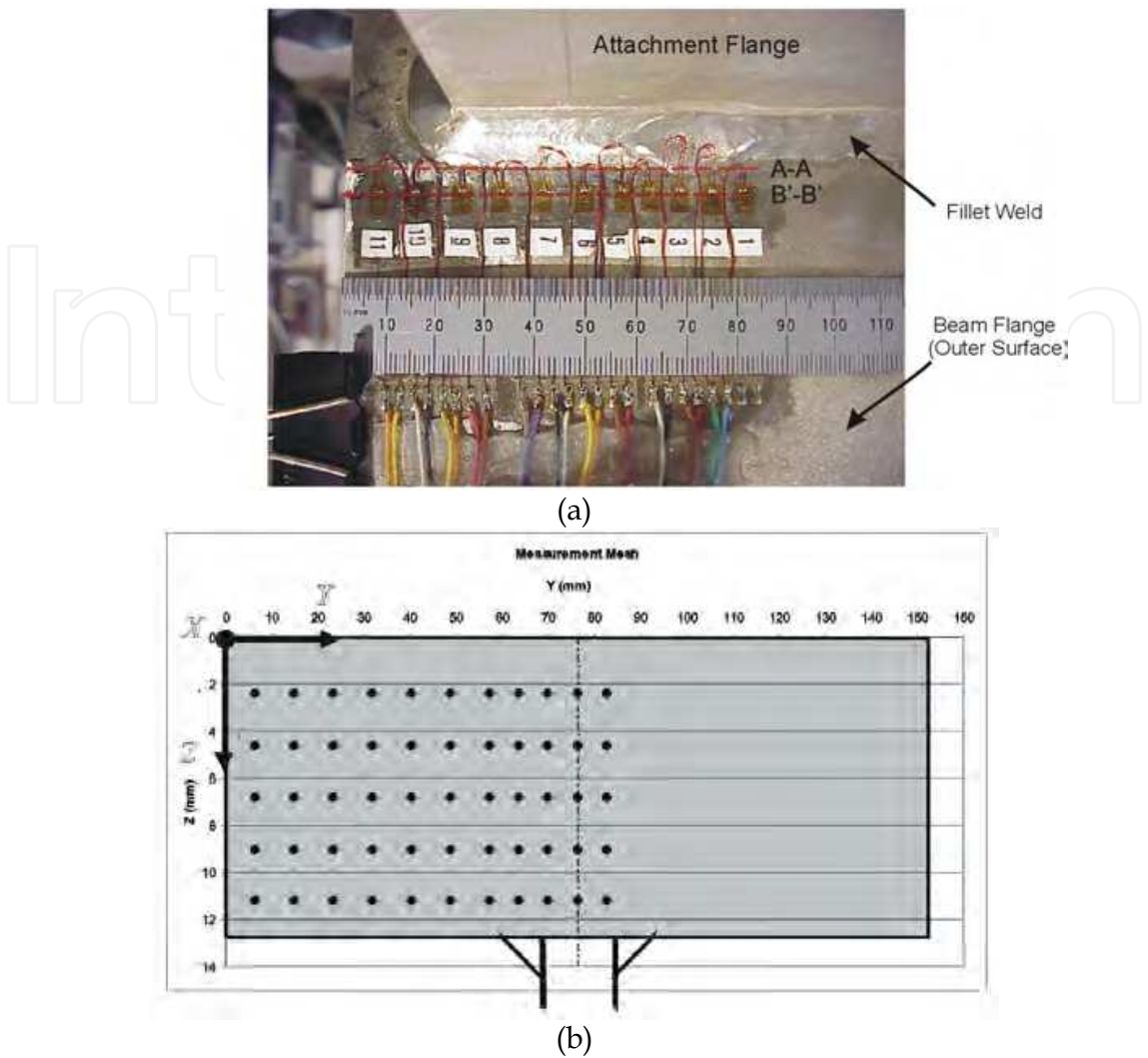
Fig. 17. Attachment welded beam segment measurement: (a)Close-up view of fillet weld for attachment welded segment; A-A plane at weld toe and B'-B' plane at 7.1 mm away from weld toe. (b) Complete measurement mesh for beam flange planes at weld toe (A-A) and 7.1 mm away from weld toe (B'-B'). Beam web centerline is at 76.2 mm (3 inch; 1 inch =25.4 mm)
