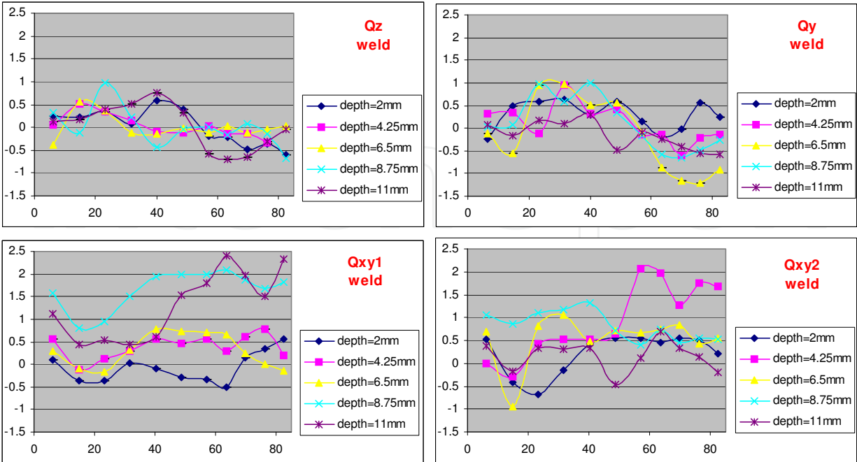
Fig. 12(a). Original strain data ( \times 10^3\mu ) for weld centerline in groove-weld segment, ( Q_{xy1} and Q_{xy2} correspond to \phi = \pm 42^\circ ; counting-statistic uncertainties are typically about \pm 0.035 ; abscissa is Y-distance from flange edge (mm; beam centerline is 76.8mm)
