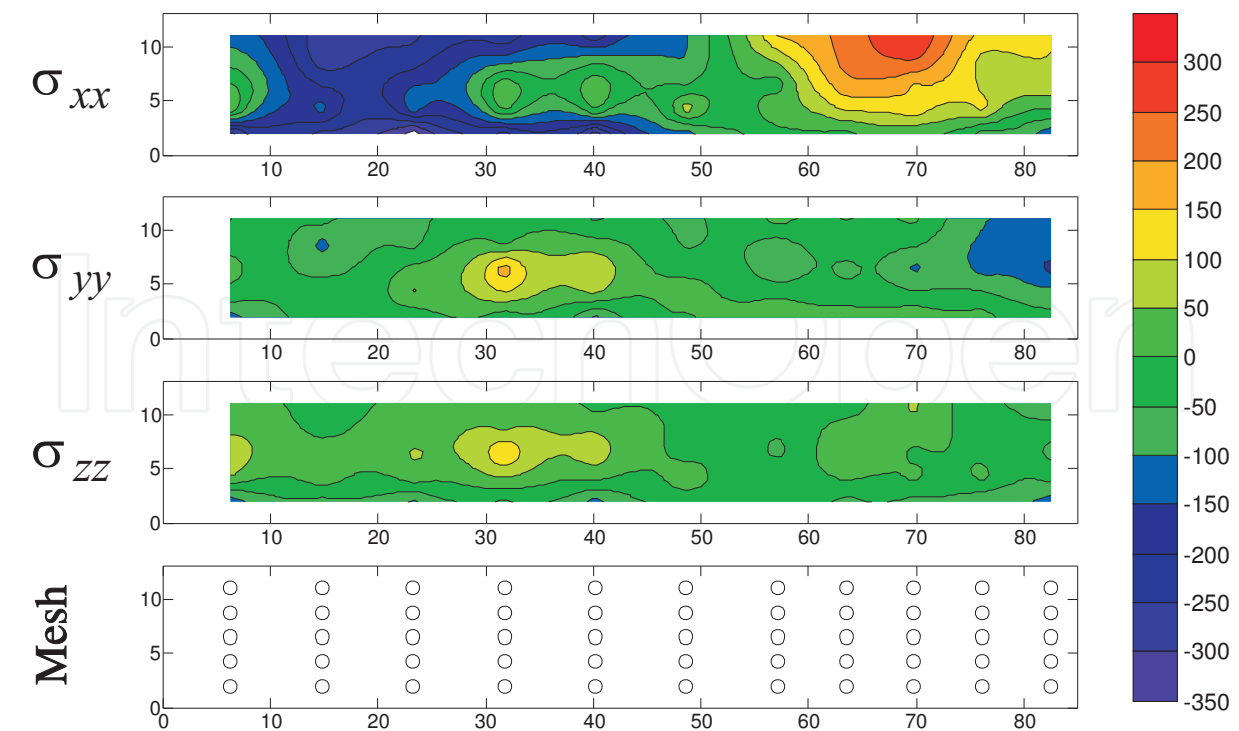
Fig. 14. Contour plots of stress data in Figure 13 for weld toe (MPa; 6.895 MPa=1ksi)
