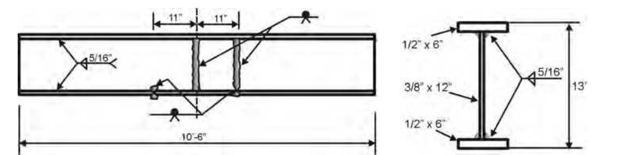
Fig. 1. Groove welded beam for residual stress measurement (unit: inch; 1 inch=25.4mm)
