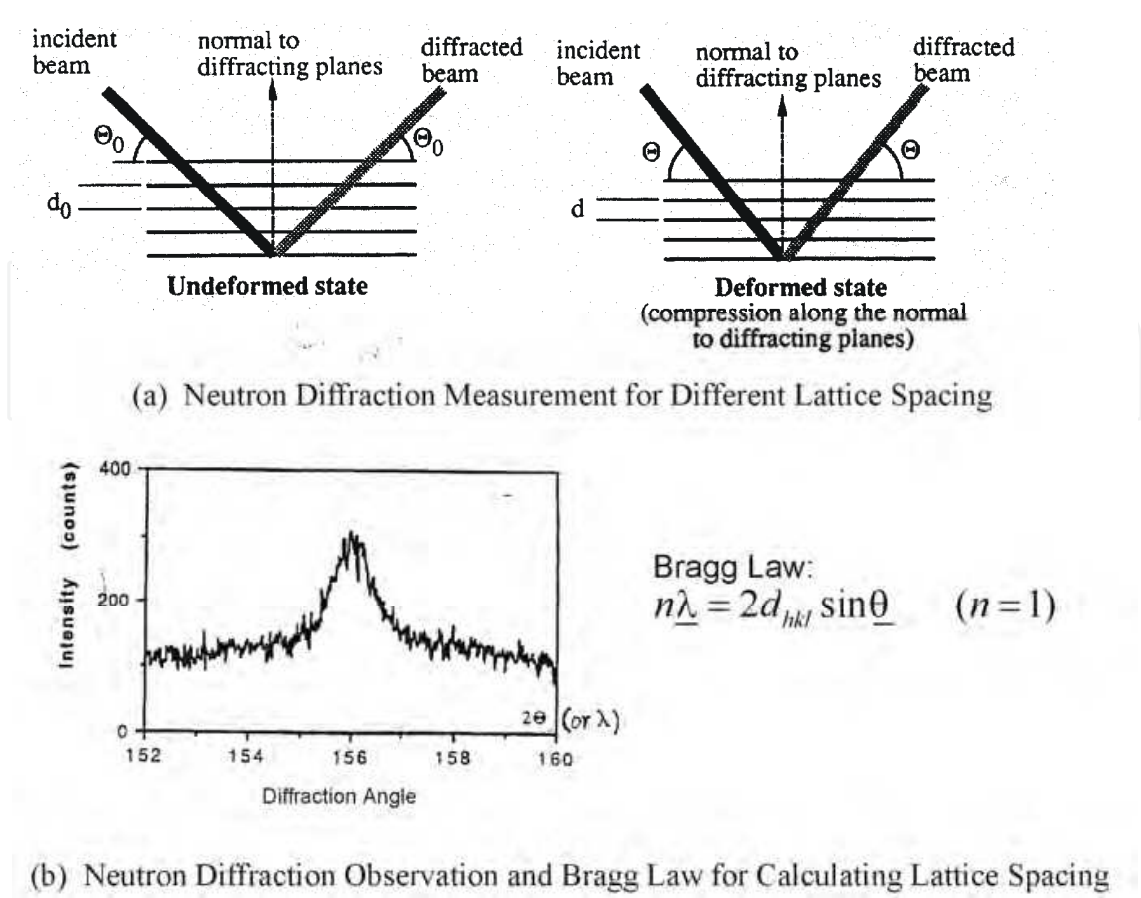
Fig. 6. Principle of neutron diffraction measurement [SEM, 1996]
