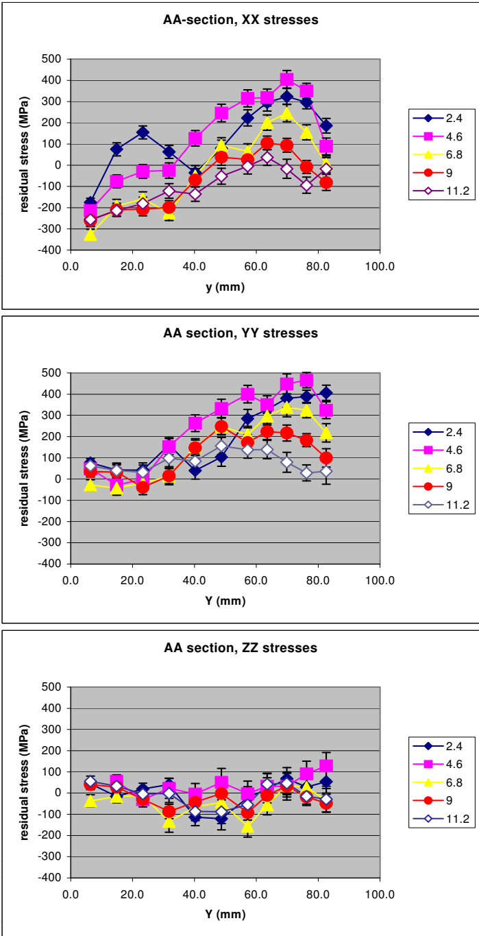
Fig. 18(a). 3-D stress data in A-A plane (weld toe) in attachment weld segment (1 ksi=6.895 MPa; beam centerline at 76.2 mm (1 inch=25.4mm))
