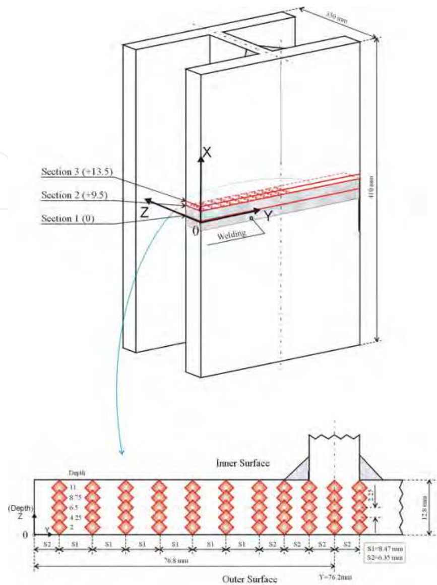
Fig. 11. Schematic measurement grid in specimen-fixed coordinate system (X-Y-Z), for groove weld segment (Unit: mm; 25.4mm=1 inch; gage volume 3x3x3mm 3 )
