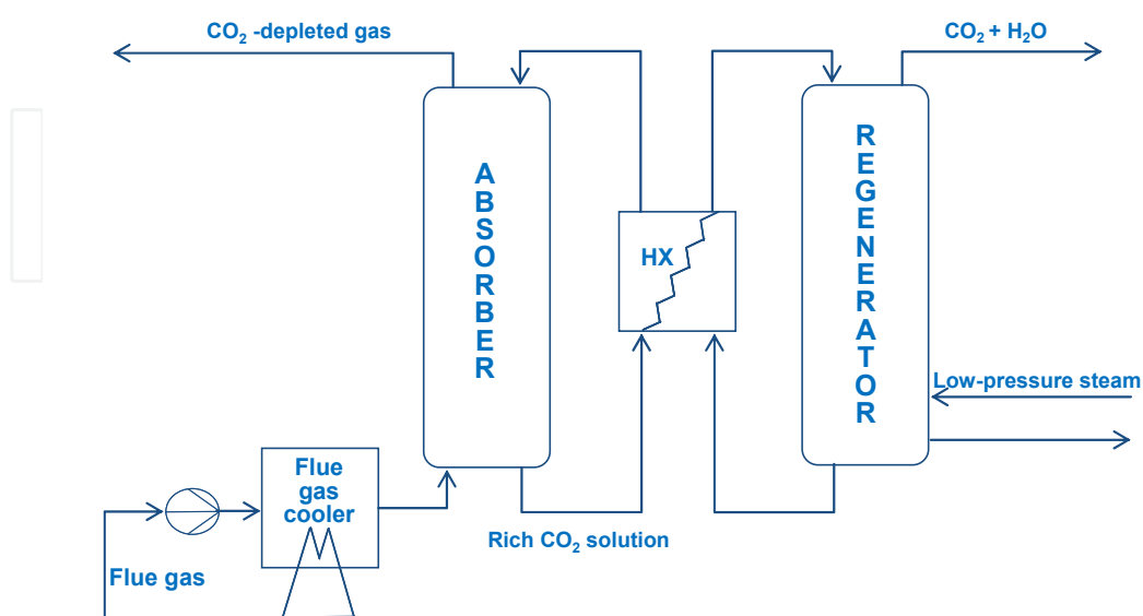
Fig. 3. Simplified diagram of a CAU.
