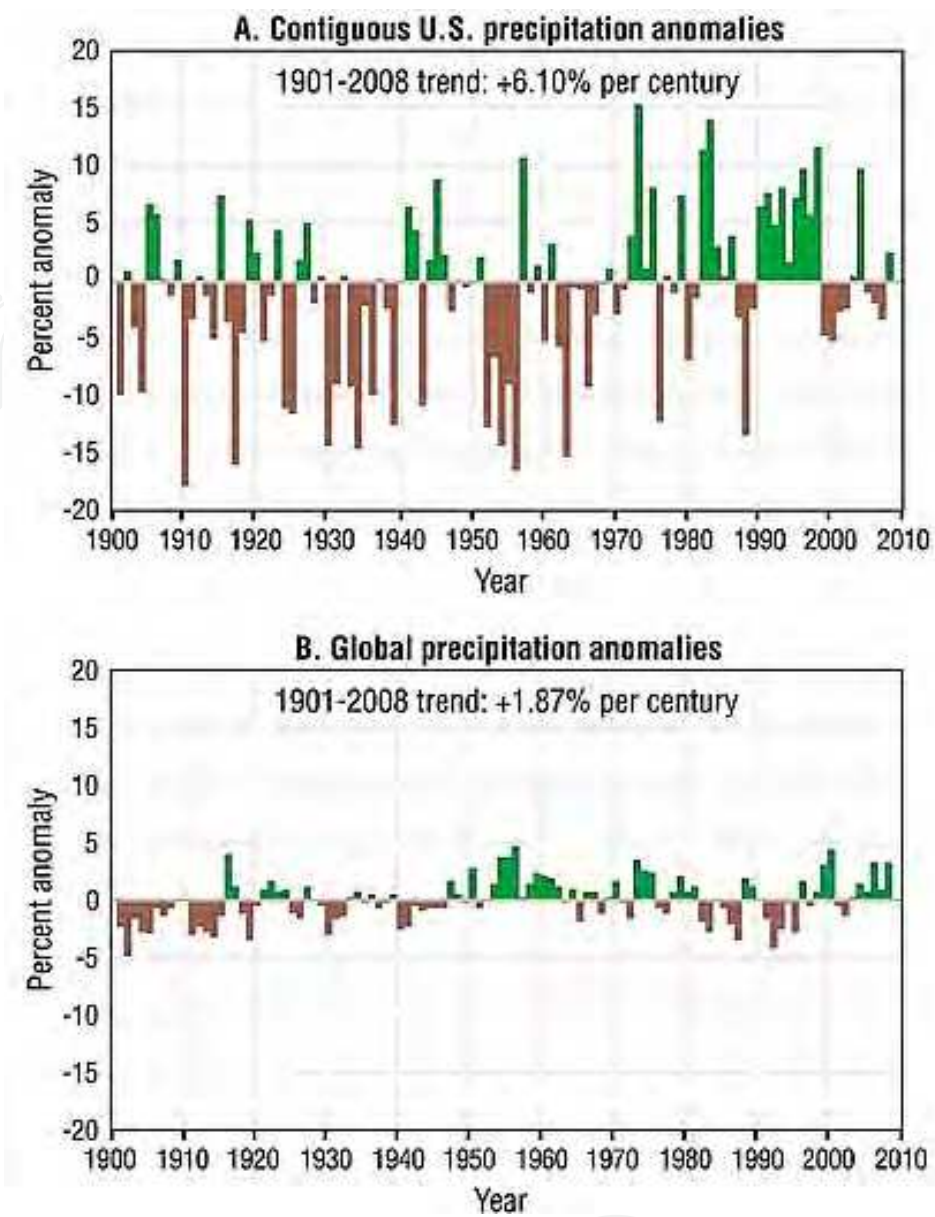
Fig. 13. Precipitation during the 20th century and up through 2008 during global warming, the NOAA estimating an observed trend over that period of 1.87% global precipitation increase per century.
