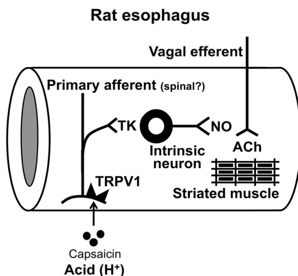
Fig. 4. Local neural reflex in the striated muscle portion of the rat esophagus. Acid as well as capsaicin can stimulate primary afferent neurons and then activate the local reflex arc. ACh; acetylcholine. TK; tachykinin. NO; nitric oxide. TRPV1; transient receptor potential vanilloid 1.
