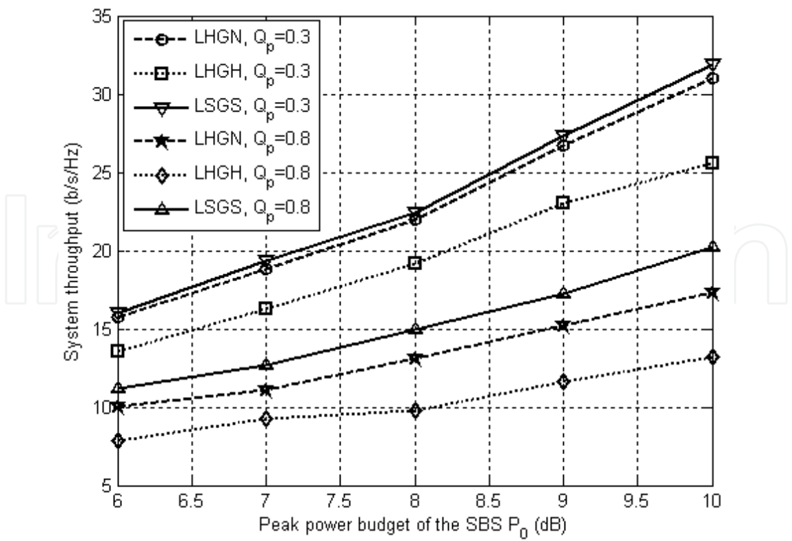
Fig. 5. System throughput versus peak power budget at K=6
