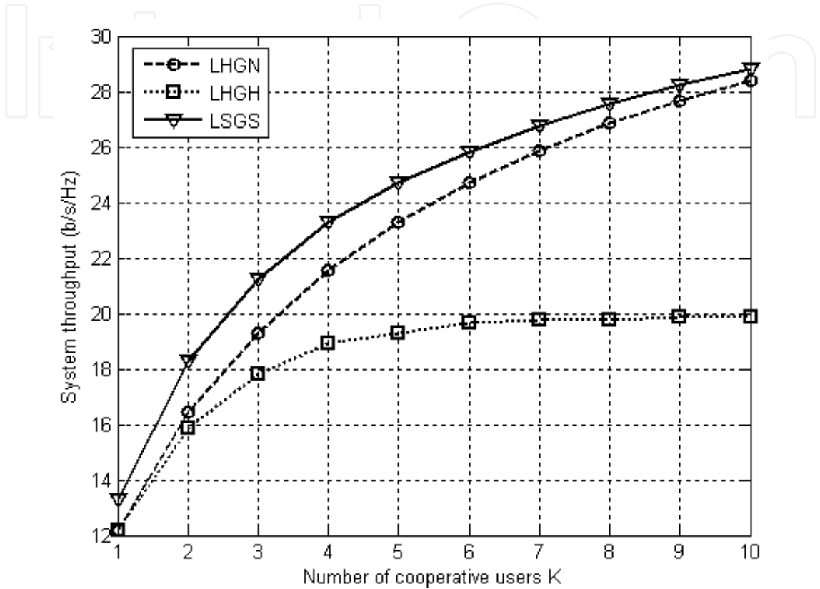
Fig. 3. System throughput versus number of cooperative users at P_0 = 10\text{dB} , Q_p = 0.5 .
