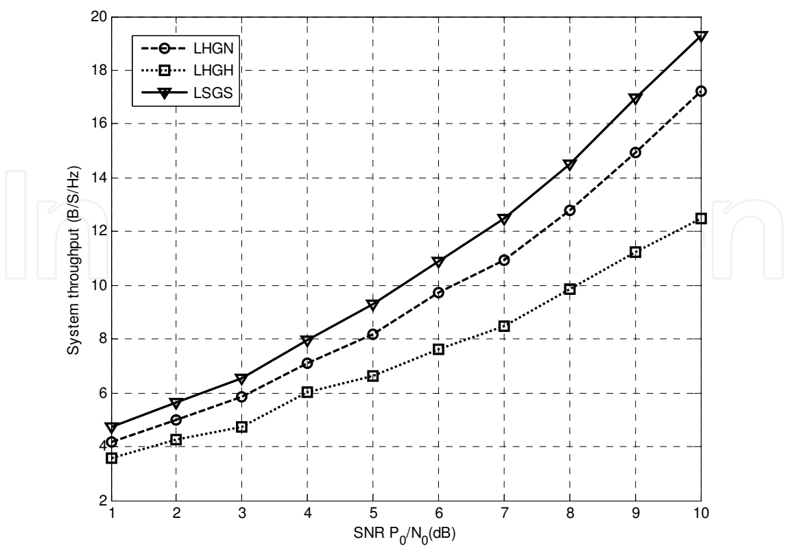
Fig. 4. System throughput versus Signal-to-Noise Ratio (SNR) at K=6
