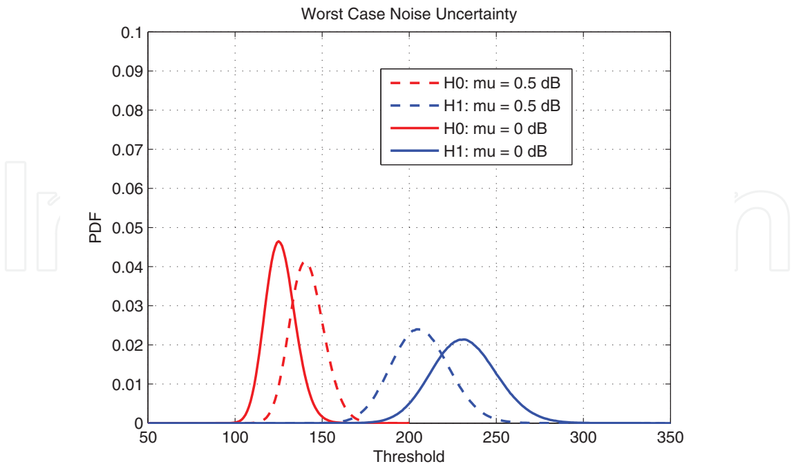
Fig. 6. Impact of worst case noise uncertainty: K = 4, N = 100, \text{SNR} = -5 \text{ dB}, \mu = 0.5 \text{ dB} .
