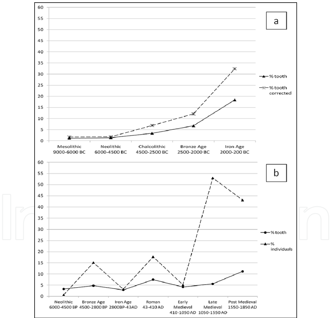
Fig. 2. Caries trends in the Old World across time. a) Indus valley civilization sequence, caries frequency versus corrected frequency (Lukacs, 1996). b) Britain sequence, caries frequency versus prevalence (Roberts & Cox, 2007).
