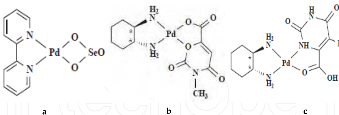
Fig. 5. The geometrical structure of [bipy]Pd(SeO 3 ) (a), [((1R,2R)-(-)-1,2-diaminocyclohexane)Pd(3-methylorotate)] (b), [(1R,2R)-(-)-1,2-diaminocyclohexane)Pd(5-fluororot) (c)] (Abu-Surrah & Kettunen, 2006)
