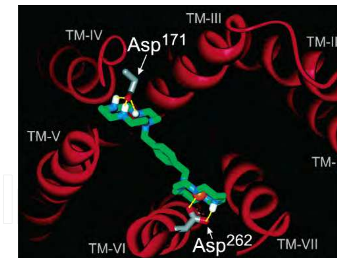
Fig. 20. Molecular model of the main ligand-binding pocket of the CXCR4 receptor with AMD3100(Zn) manually docked into favorable interactions with Asp171 in TM-IV and Asp262 in TM-VI. The receptor model is built over the rhodopsin model of Palczewski et al (Palczewski et al, 2000). The conformation of AMD3100 is based on structural requirements of high antiviral effects of AMD3100 and the crystallographic X-ray structure of 6,6'-spirobis- (1,4,8,11-tetraazacyclotetradecane)-dinickel(II)tetraperchlorate, obtained from the Cambridge Structural Database (Gerlach et al, 2003).
