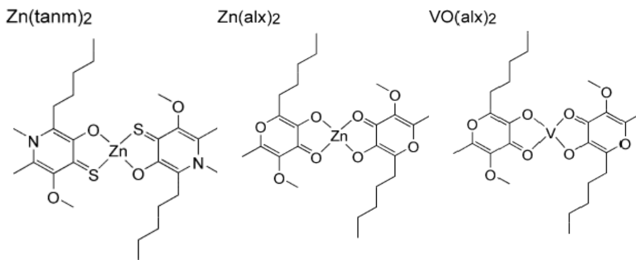
Fig. 21. The molecular structures of \text{VO}(\text{alx})_2 , \text{Zn}(\text{alx})_2 , and \text{Zn}(\text{tanm})_2 (Hiromura & Sakurai, 2008)
