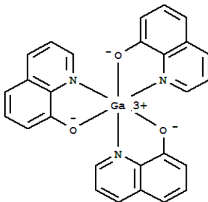
Fig. 9. Molecular structure of Tris(8-quinolinolato)gallium(III)
