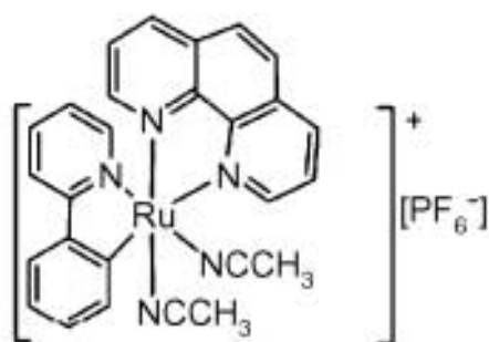
Fig. 8. Molecular structure of RDC11 (Meng et al, 2009).
