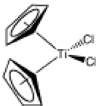
Fig. 10. Molecular structure of titanocene (Hannon, 2007)
