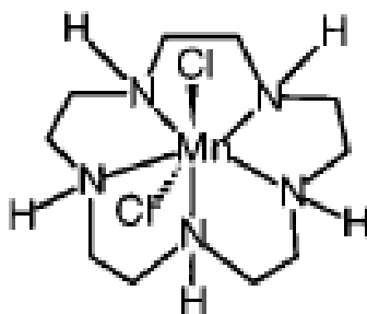
Fig. 15. Molecular structure of SC-52608 (Guo & Sadler, 1999)
