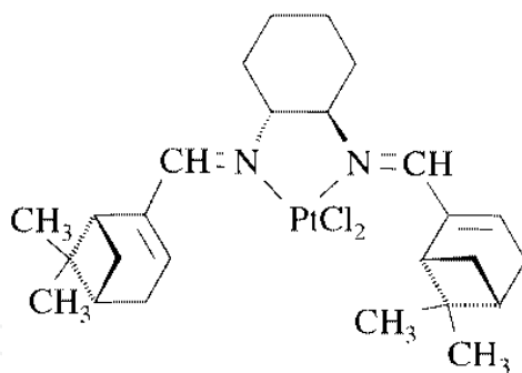
(a) Dichloro[(1R,2R)-(-)-N 1 ,N 2 -bis{(1R)-(-)-myrtenyl}-1,2-diamino cyclohexane]-platinum(II).3H 2 O
