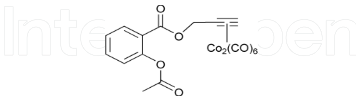
Fig. 18. The structure of hexacarbonyldicobalt-aspirin complex (Ott et al, 2009)
