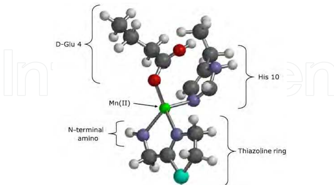
Fig. 17. \text{Mn(II)} ligand models derived from metallobacitracin complexes (Piacham et al, 2006)
