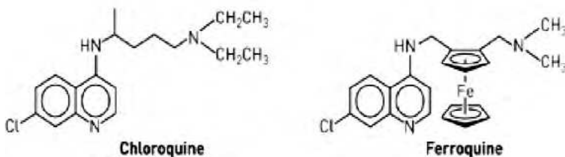
Fig. 14. Molecular structure of Chloroquine and Ferroquine.
