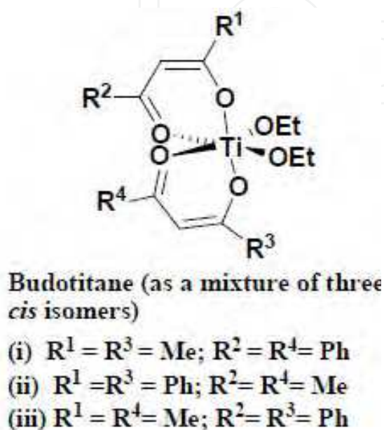
Fig. 11. The molecular structure of budotitane (Bharti & Singh, 2009).
