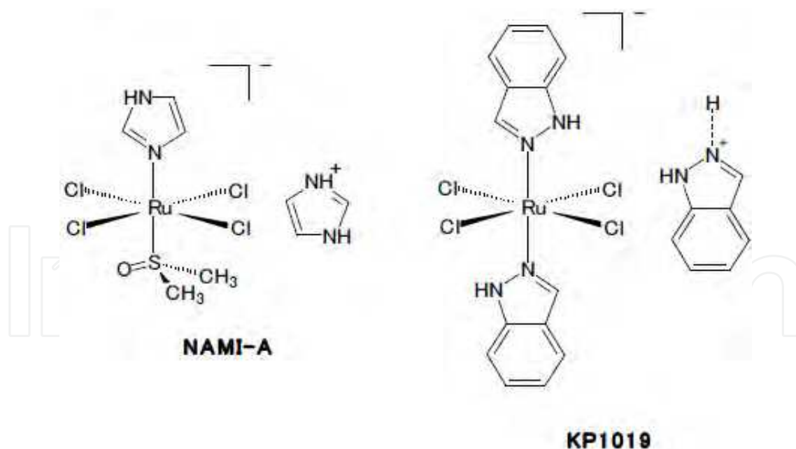
Fig. 7. Structure of ruthenium complexes NAMI-A and KP1019 (Llorca, 2005).
