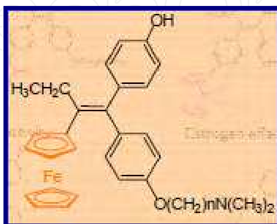
Fig. 6. The main molecular structure of ferrocifenes.
