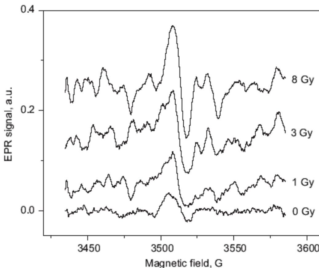
Fig. 11. EPR Spectra of fingernails treated with dithiothritol for 20 min after receiving different radiation doses (Romanyukha , a., et al., 2007).
