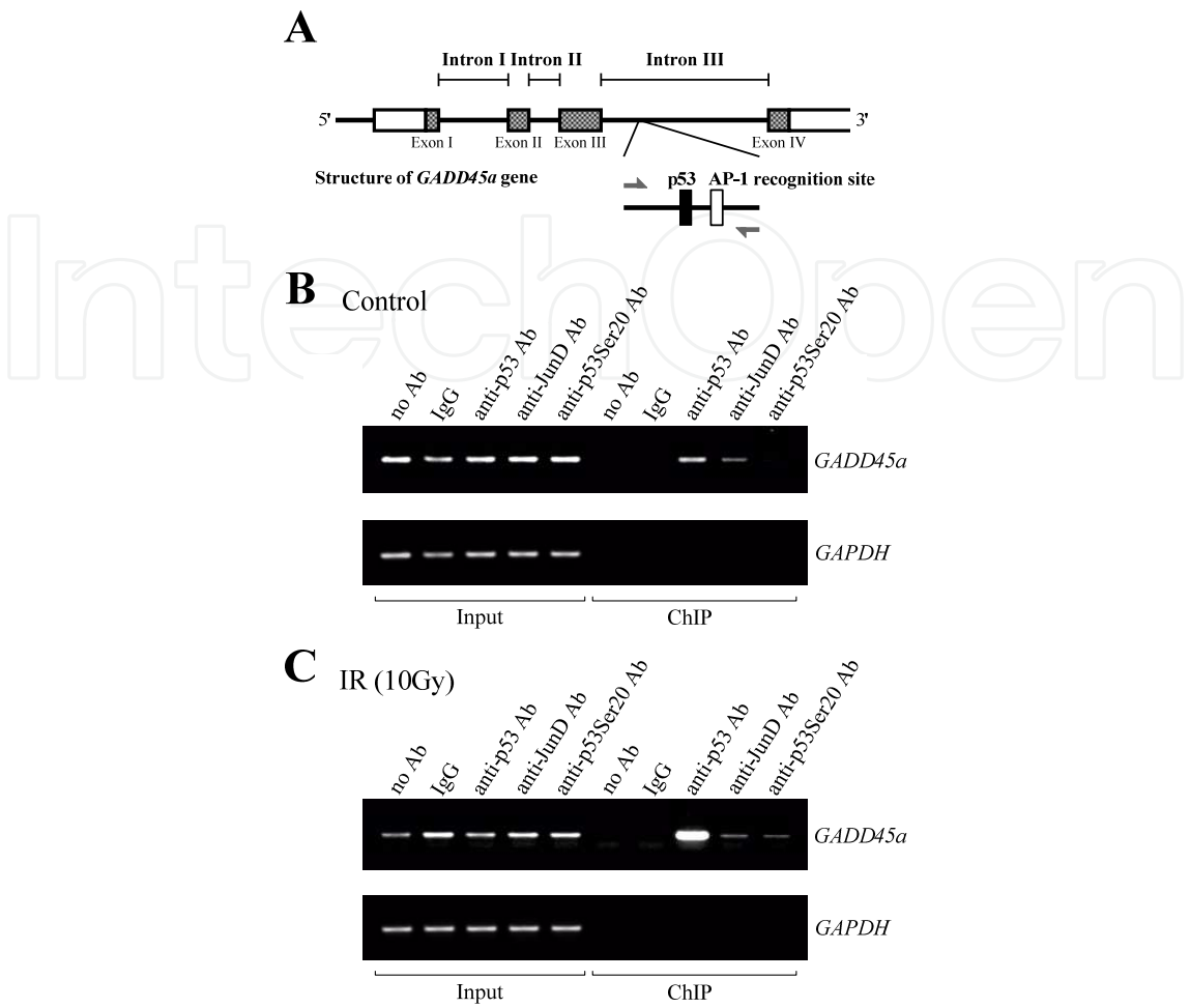
Fig. 10. Chromatin immunoprecipitation (ChIP) analysis for the in vivo binding of JunD at the third intron. (A) Schematic illustration of genomic structure of the GADD45A gene. PCR primers were designed to amplify the region containing both the p53 site and the AP-1 site, as represented by arrows. (B) ChIP analysis was performed with MCF-7 cells, unirradiated (B) or exposed to 10 Gy of X-rays with 1.5 h postincubated (C). Sheared chromatin was incubated without antibodies (no Ab) or with the IgG, anti-p53 antibody, anti-JunD antibody, and anti-phospho-p53 (Ser20) antibody. Immunoprecipitants were analyzed by PCR. The GAPDH promoter containing neither an AP-1 nor p53 site was analyzed as a negative control. PCR was performed for 32 cycles, which was in the linear range of amplification, except for the case using the sample prepared from X-ray-treated cells with the anti-p53 antibody. (Reproduced with permission of Elsevier B. V. from Ref (Daino et al., 2006))
