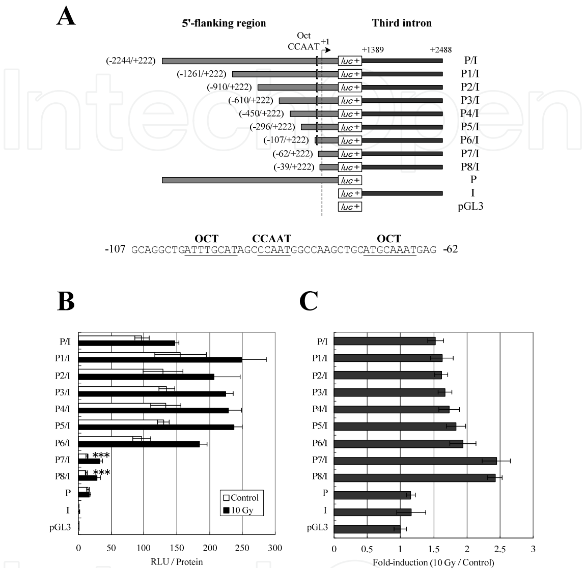
Fig. 8. Reporter gene analysis for the promoter activity of the GADD45A gene. (A) Various GADD45A -luciferase constructs are schematically illustrated. The light gray bars and the dark gray bars represent the 5'-flanking region and the third intron region of the GADD45A gene, respectively. The transcription start site is indicated by an arrow. The nucleotide sequence of the region, which reduced the basal promoter activity significantly as shown in (B), is presented at the bottom. Two OCT sites and a CCAAT box are underlined. (B) MCF-7 cells transiently transfected with reporter constructs were either irradiated with 10 Gy of X-rays (closed bars) or mock-treated as a control (open bars), and the luciferase activity in the cell lysates prepared 5 h after irradiation was measured. The relative light unit (RLU) per protein concentration is plotted. (C), Fold-induction of the luciferase activity after irradiation with 10 Gy of X-rays is plotted. Results are the mean of at least three independent experiments. Error bars represent the S.D. (***) p < 0.001 versus P/I, student's t-test). (Reproduced with permission of Elsevier B. V. from Ref (Daino et al., 2006))
