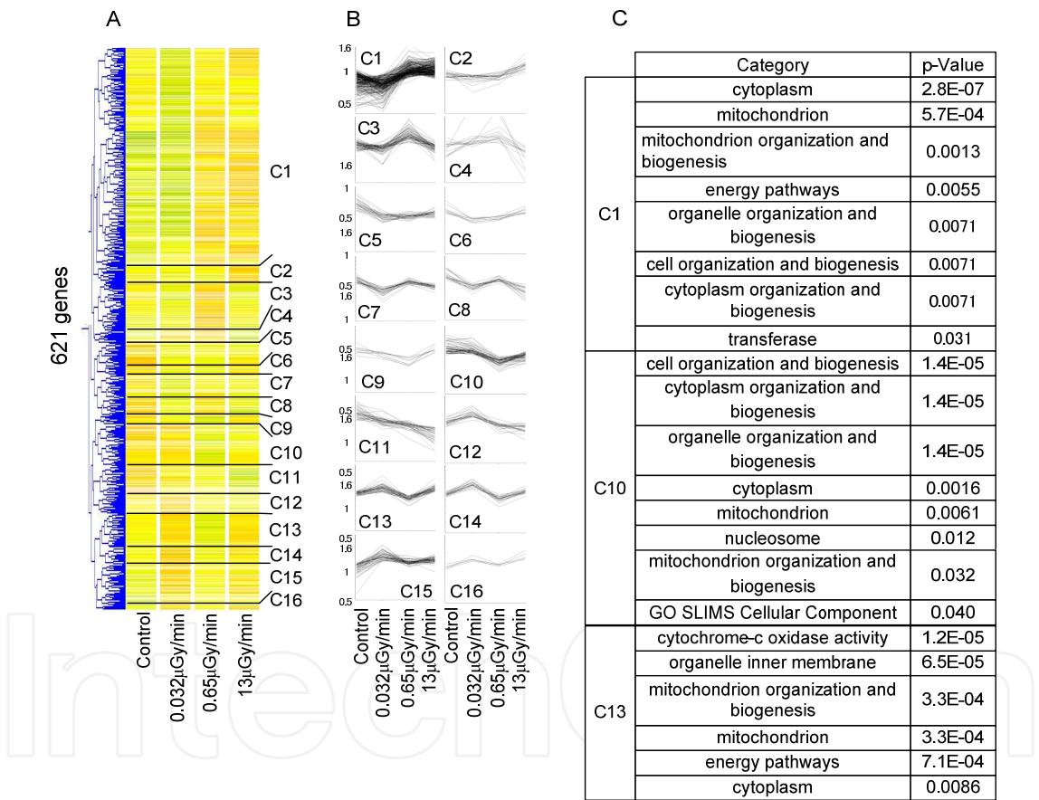
Fig. 15. Hierarchical cluster analysis of genes whose expression was modulated after irradiation with a statistical significance in the kidney. A: Expression levels of 621 of significantly modulated genes are indicated by color. Green, yellow, and red colors represent low, medium, and high expression, respectively. On the basis of the expression pattern, genes were classified into 16 clusters. B: Expression profiles of genes in each of the 16 clusters are collectively shown. C: Gene Ontology categories significantly overlapped with the gene clusters are shown. No Gene Ontology categories significantly similar to the clusters other than C1, C10 and C13 were found. (Reproduced with permission of the Japanese Radiation Research Society from Ref (Taki et al., 2009))
