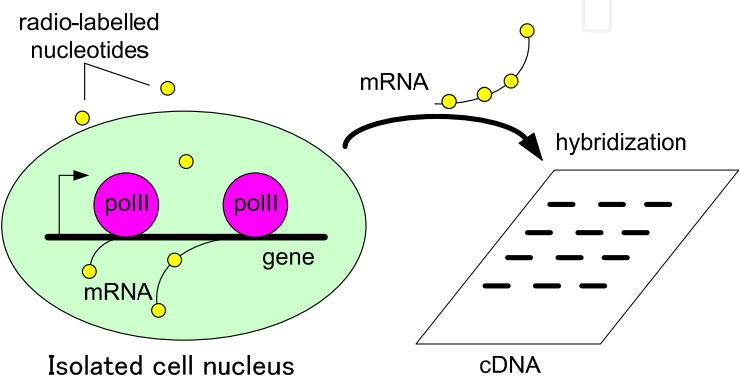
Fig. 2. Schematic illustration of the nuclear run-on assay.
