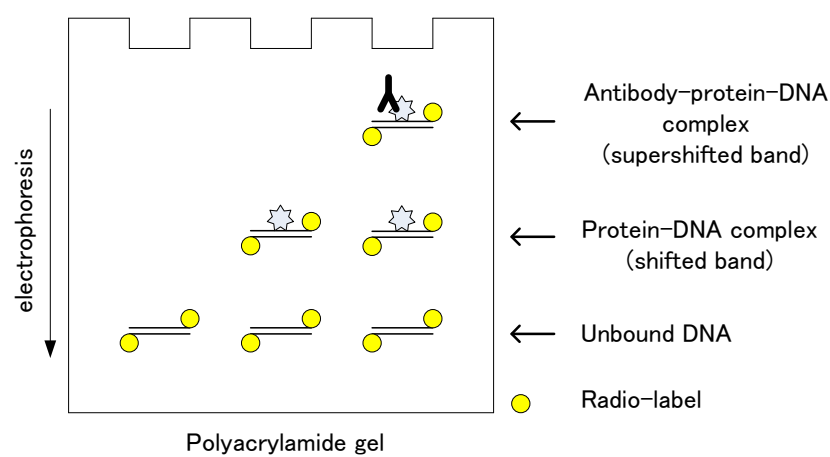
Fig. 4. Scematic illustration of electrophoretic mobility shift assay (EMSA)
