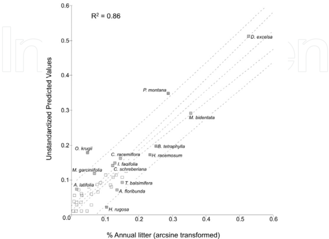
Fig. 2. Stepwise regression model for % annual litterfall (as the dependent variable) and importance values of vegetation for height class >10 m and crown area class >25 m 2 (as the independent variables). Unstandardized predicted values were obtained using SPSS 2002, version 11.5, Chicago, Illinois, USA. Refer to Table 1 for complete species names.
