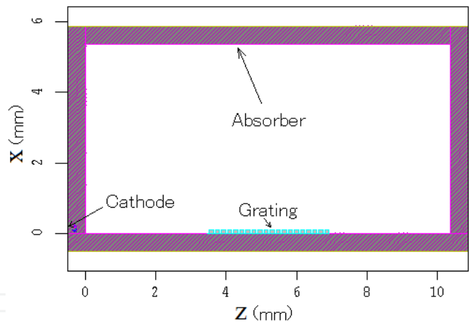
Fig. 5. Geometry used in simulation. (The surface of the grating is assumed to consist of a perfect conductor)
