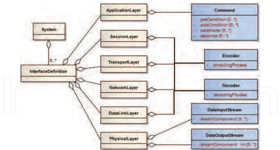
Fig. 9. Overview of SID extension to SensorML.
