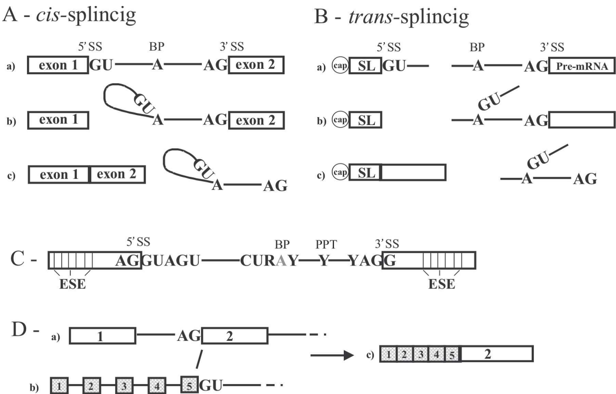
Fig. 4. Schematic representation of cis- and trans-splicing pathways.
