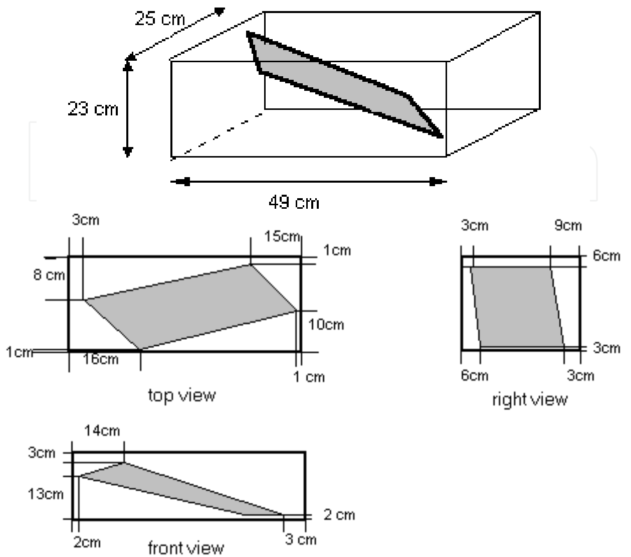
Fig. 3. Prepared concrete block and the dimension of the surface
