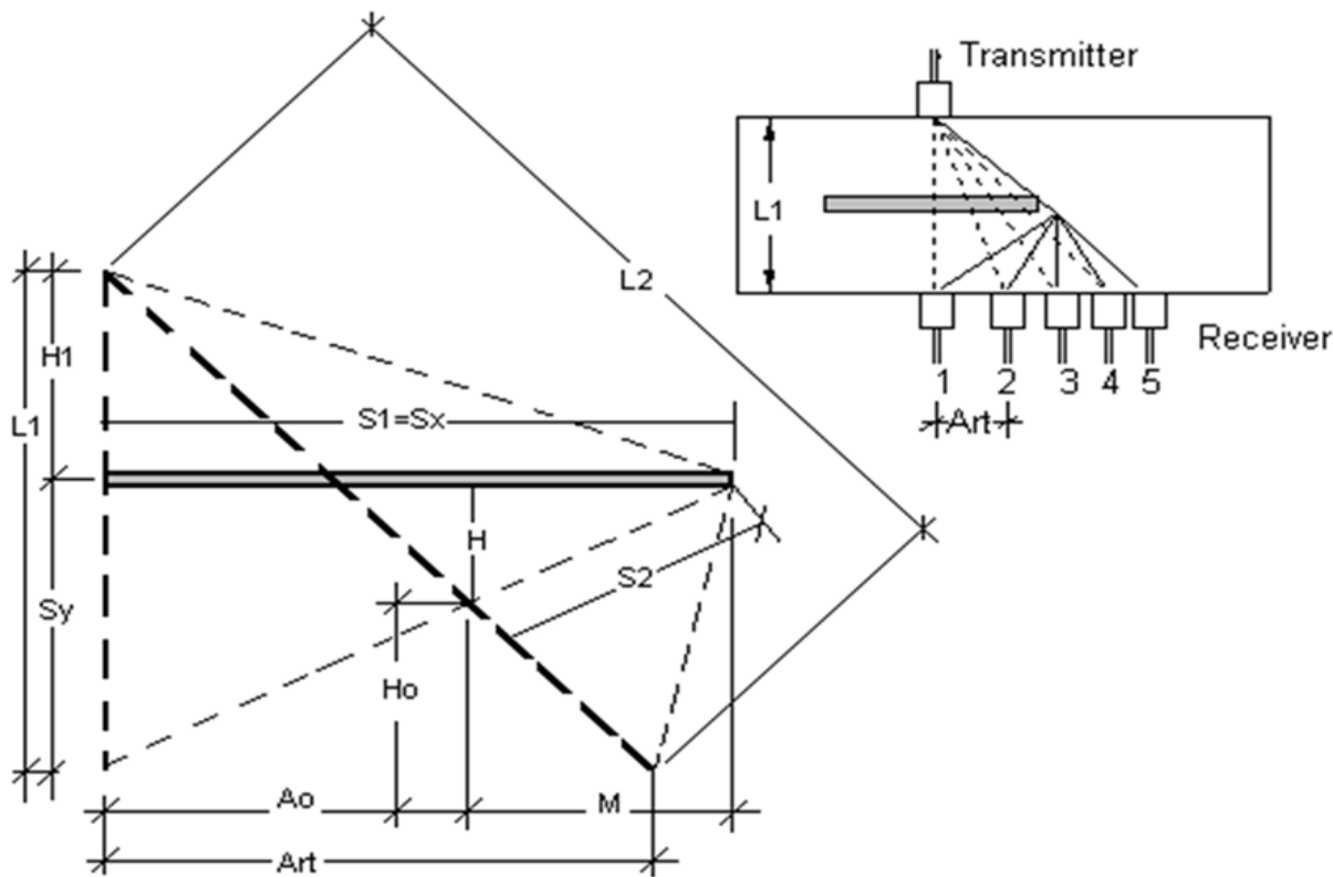
Fig. 13. Pulses travel paths for both receiver positions.
