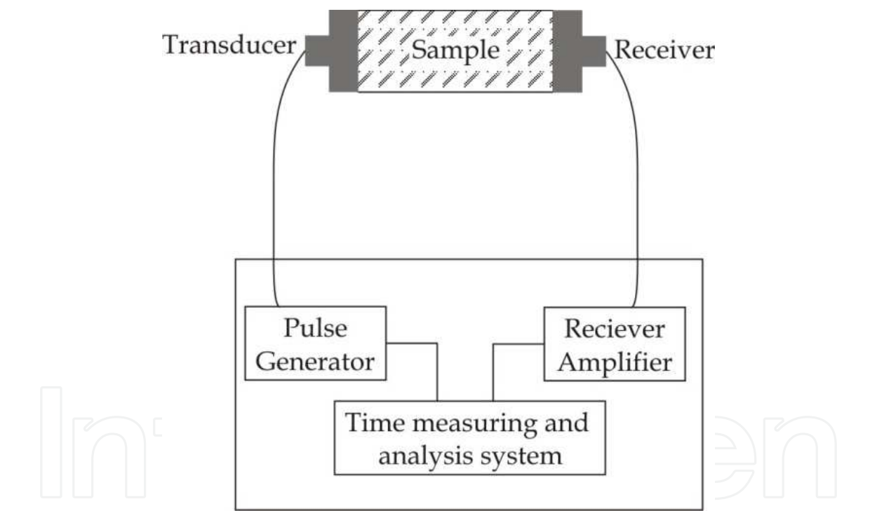
Fig. 1. Pulse velocity test (Malhotra & Carino, 1991)
