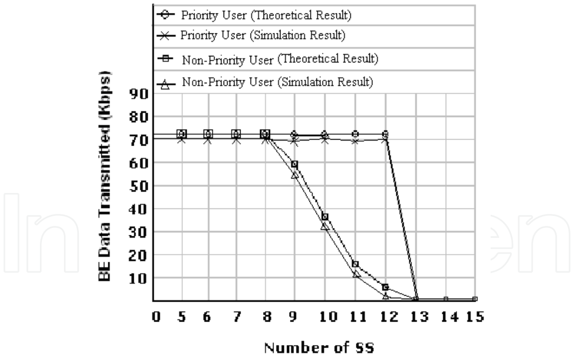
Fig. 12. BE data (in Kbps) transmitted by priority-SS compared to regular-SS.
