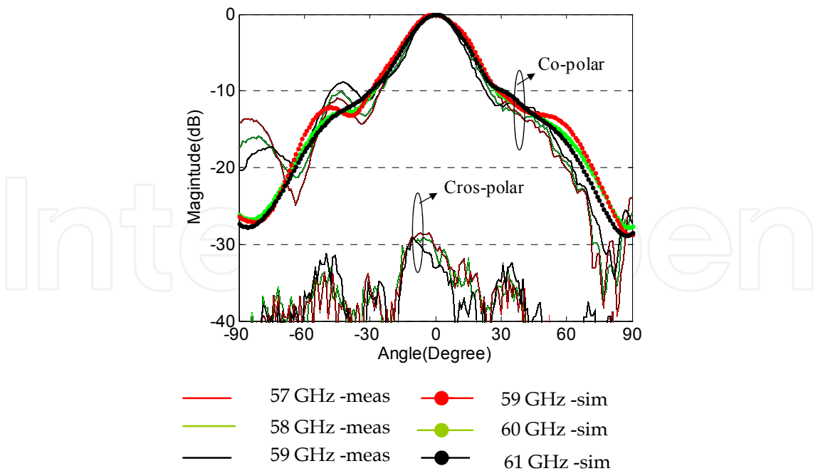
Fig. 10a. Measured and simulated E-plane radiation patterns of superstrate antenna.
