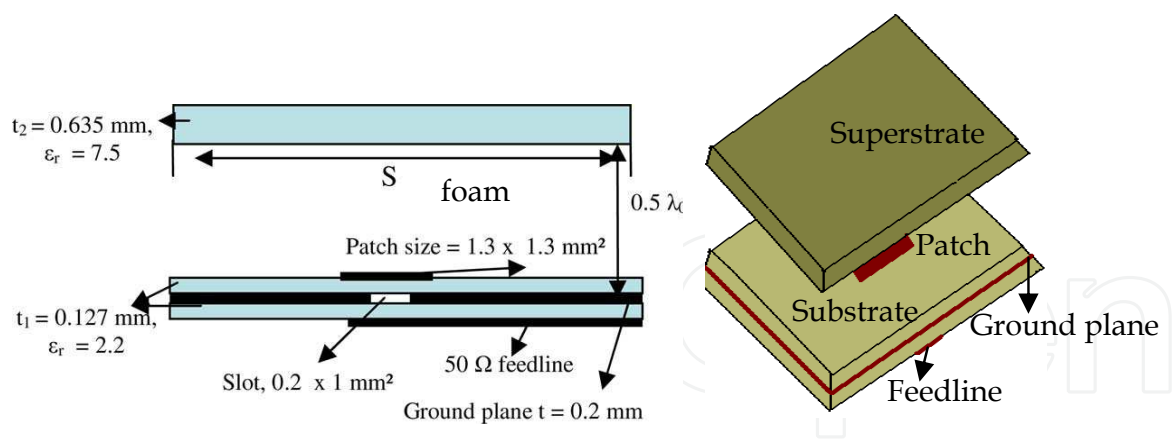
Fig. 7. Cutting plane and 3D view of aperture coupled antenna with superstrate, ground plane size = 30 x 30 mm².
