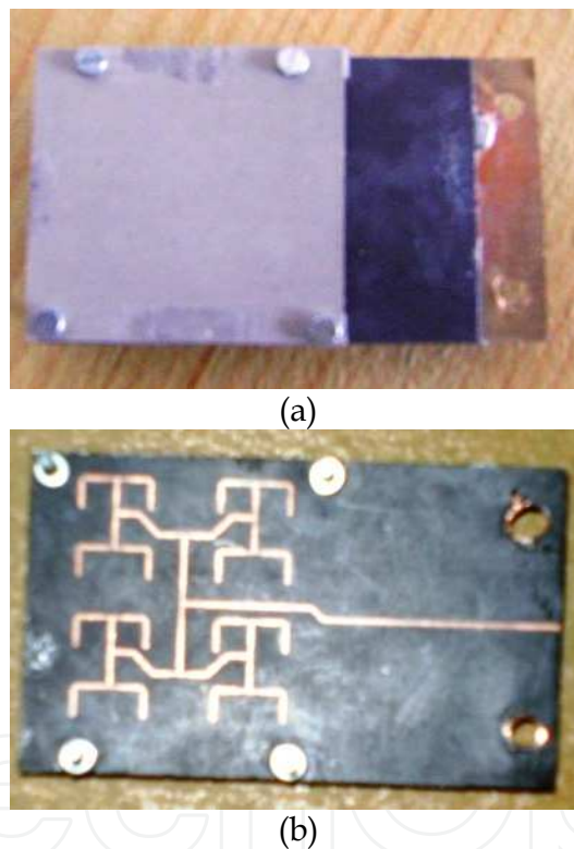
Fig. 17. Photograph of 4 \times 4 superstrate antenna array prototype (a) Top view of superstrate antenna (b) view of antenna feed line network from bottom side. Ground plane taken is 6\lambda_0 \times 10\lambda_0 , for connecting V band connector and for ease of measurement purpose.
