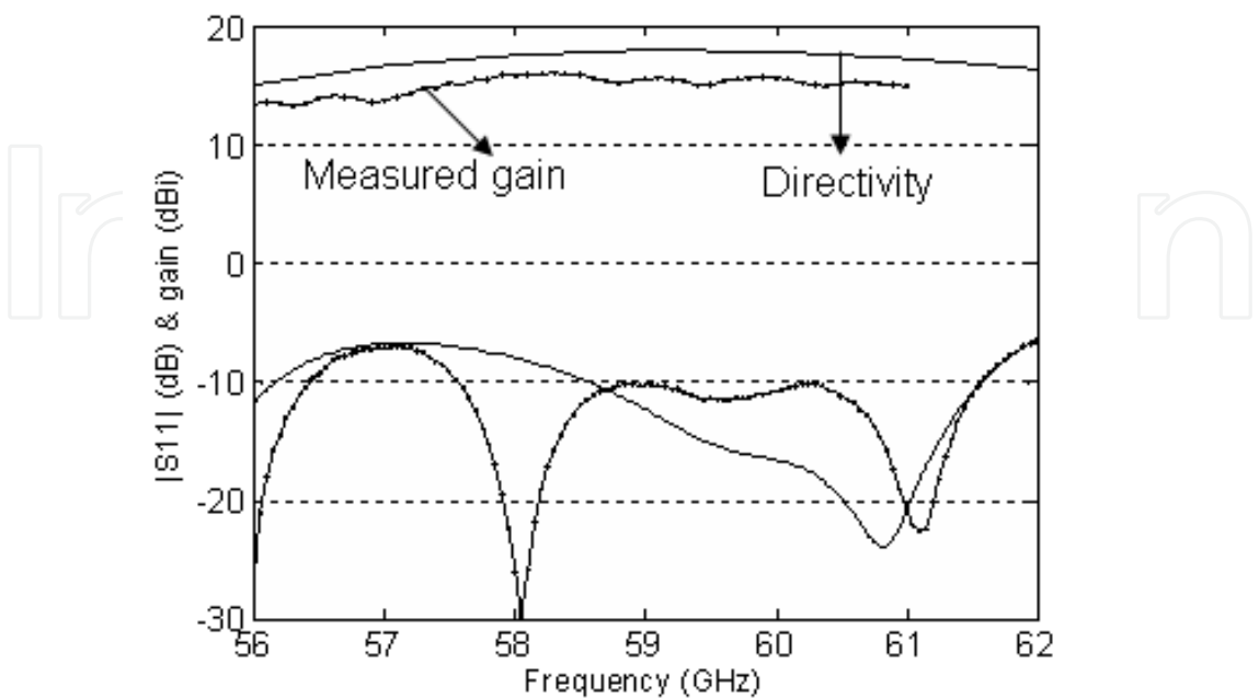
Fig. 14. Variation of S11 and gain with a superstrate dimension of 3.2 \lambda_0 . Simulation ——— measured —•— .
