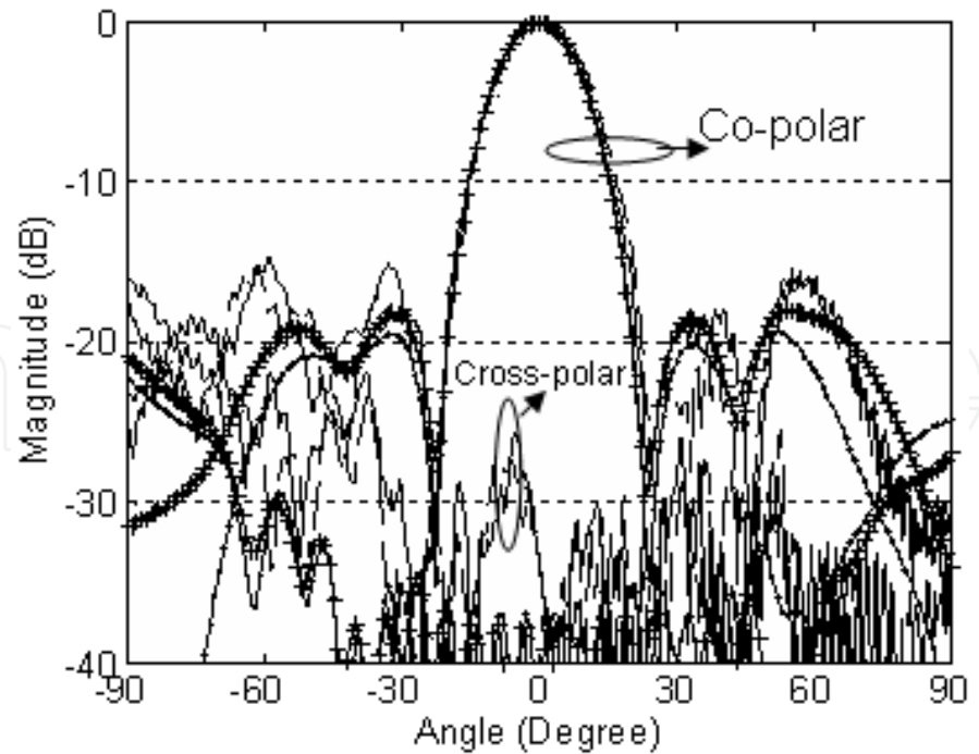
Fig. 16. Measured and simulated H-plane radiation patterns of 2 x 2 superstrate antenna array. 58 GHz - measured --- 59 GHz - simulated —•— 59 GHz - measured — 60 GHz - simulated —+— .
