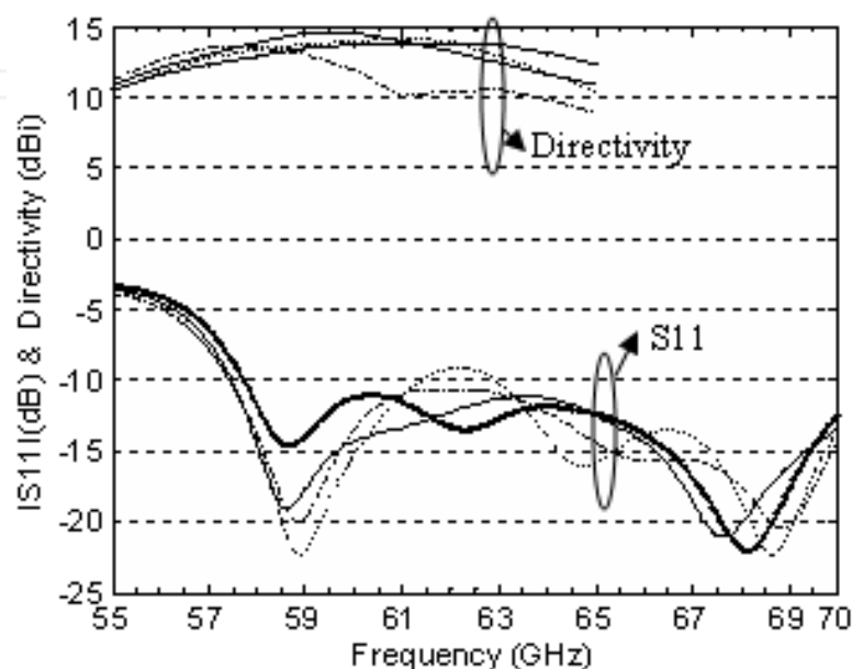
Fig. 22. Simulated results of S11 and directivity with various superstrate dimensions. 1\lambda_0 \times 2\lambda_0 —•— ; 2\lambda_0 \times 2\lambda_0 ..... ; 1.2\lambda_0 \times 2.7\lambda_0 — ; 3\lambda_0 \times 3\lambda_0 - - - - .
