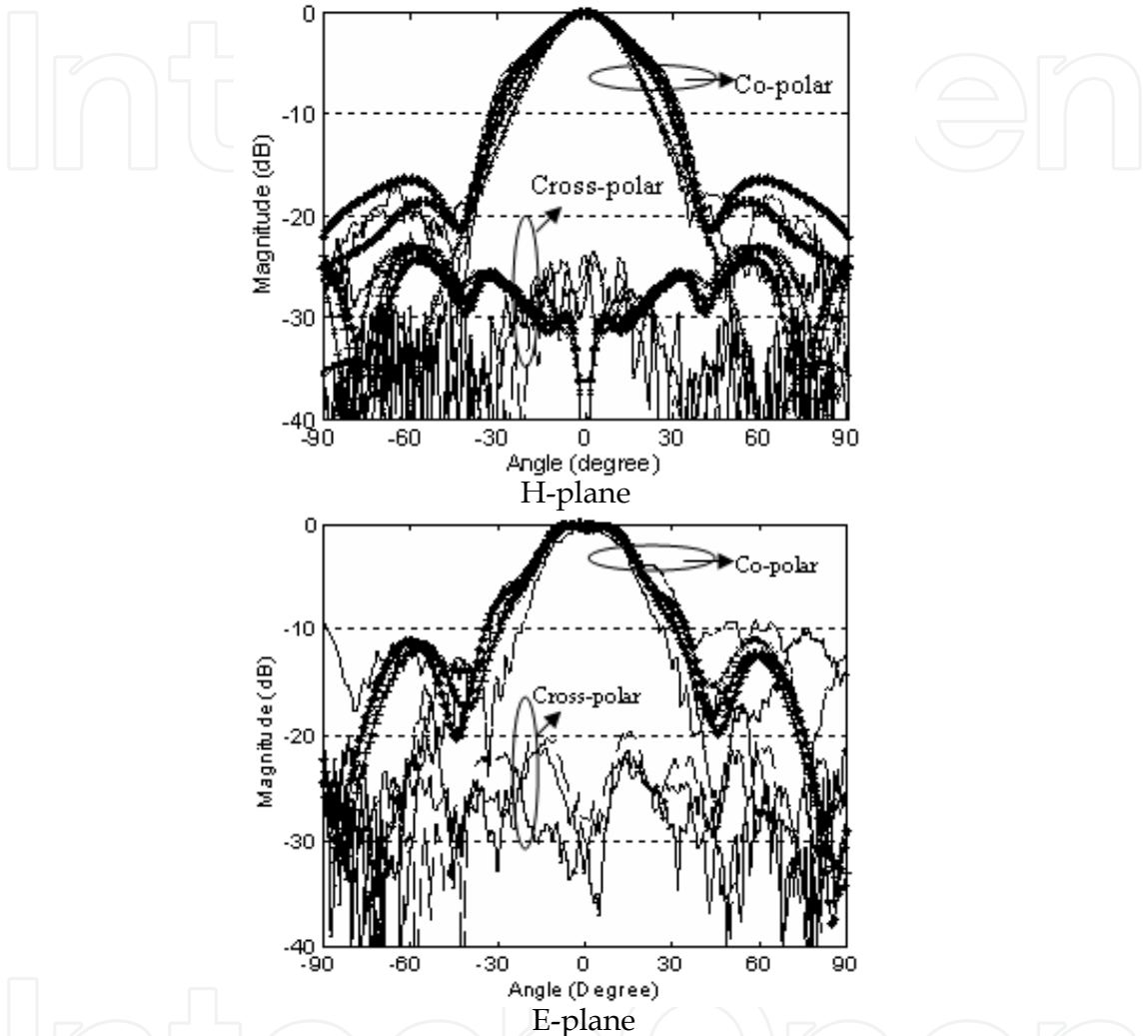
Fig. 24. Measured and simulated H-plane & E- plane radiation patterns of superstrate antenna (Co and Cross polarisation).
