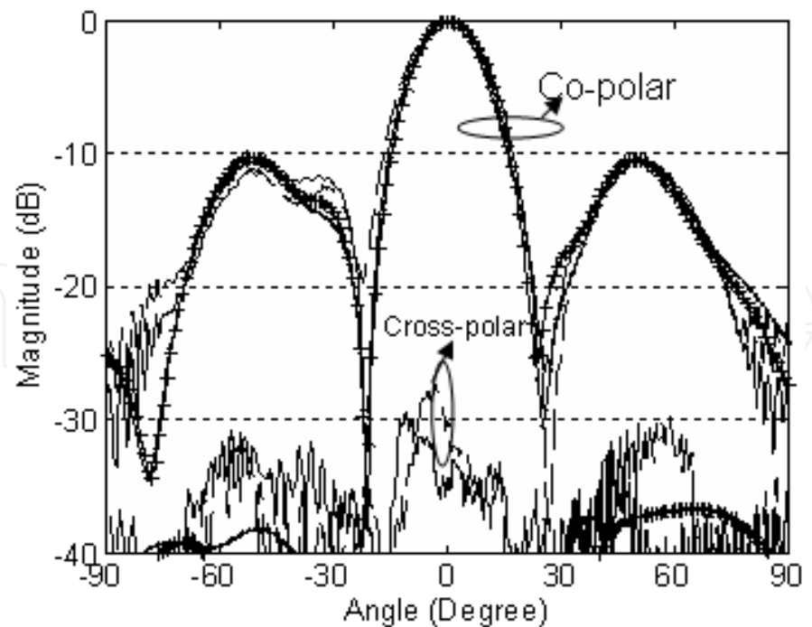
Fig. 15. Measured and simulated E-plane radiation patterns of 2 x 2 superstrate antenna array. 58 GHz - measured --- 59 GHz - simulated —•— 59 GHz - measured — 60 GHz - simulated —+— .
