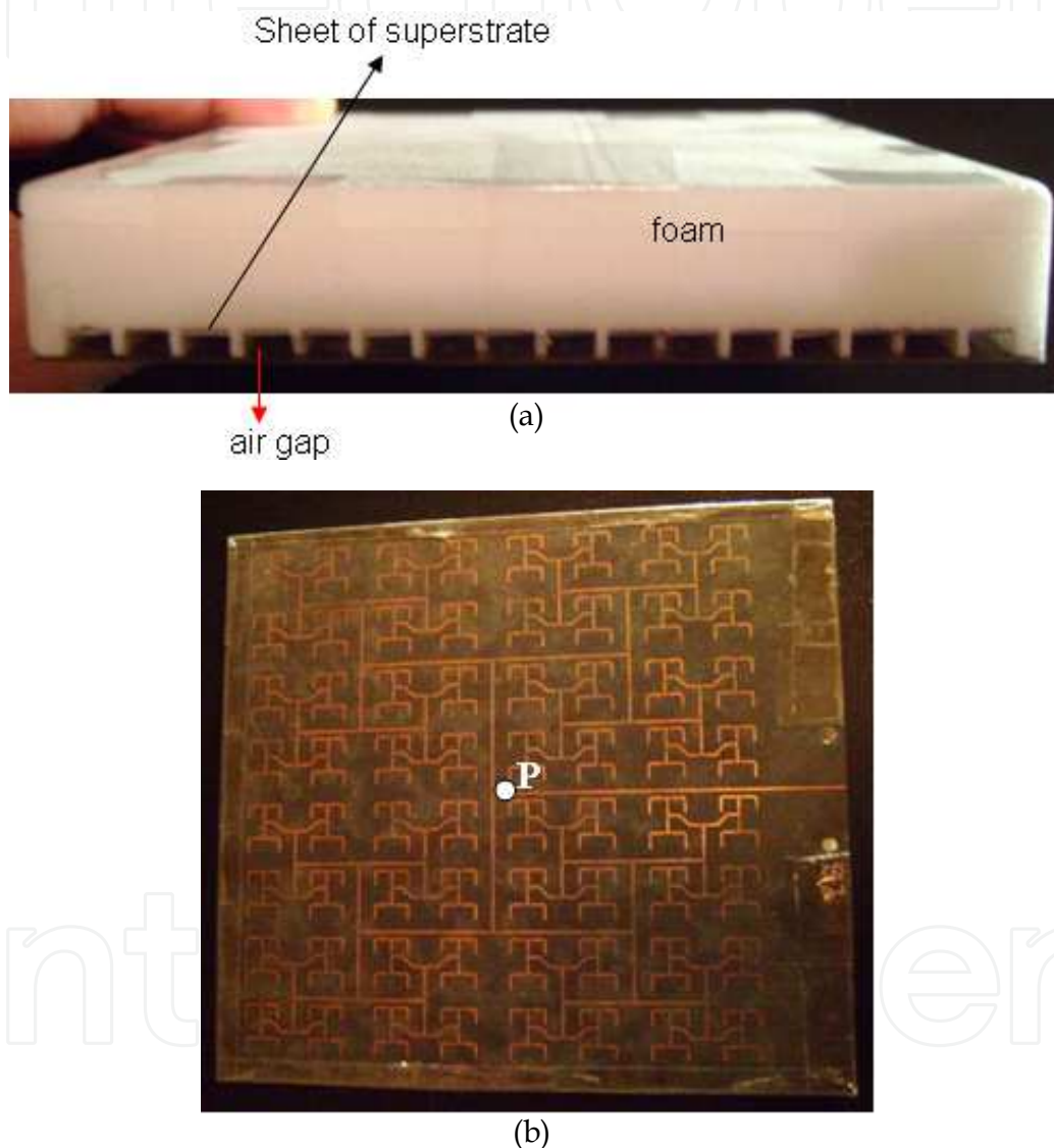
Fig. 29. (a) Side overview of 16 \times 16 array prototype: details of the 16 separate superstrate sheets and air gap within foam, total size = 20.6 \lambda_0 \times 21.8 \lambda_0 . (b) 16 \times 16 feed network.
