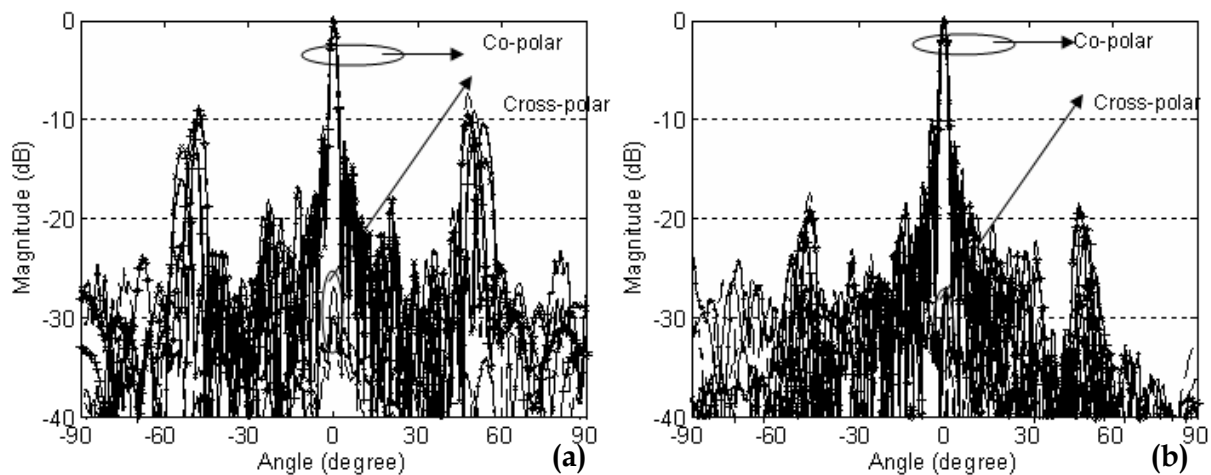
Fig. 31. Measured and simulated E-plane (a) & H-plane (b) radiation patterns of the 2 x 2 superstrate antenna array (Co and Cross polarisation). 57 GHz - Simulated —×— ; 57 GHz - Measured —•— ; 60 GHz - Simulated —+— ; 60 GHz - Measured — — — ; 62 GHz - Simulated —*— ; 62 GHz - Measured — — — .
