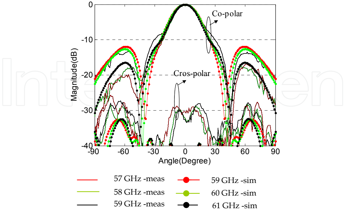
Fig. 10b. Measured and simulated H-plane radiation patterns of superstrate antenna.
