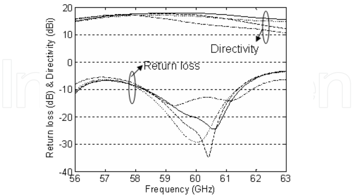
Fig. 13. Variation of return loss and directivity with various superstrate dimensions. 2.4 \lambda_0 ..... 3.2 \lambda_0 — 4 \lambda_0 ---- 6 \lambda_0 - · - · - .
