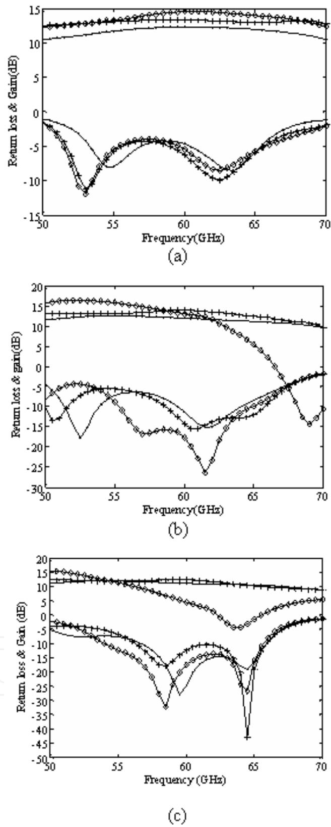
Fig. 3. variation of s11 and gain with superstrate dimension and height from ground plane. a) h_2=0.5\lambda_0 b) h_2=0.6\lambda_0 c) h_2=0.7\lambda_0 for size =.73\lambda_0 —●— size =1.1\lambda_0 —+— size =2\lambda_0 —◇— .
