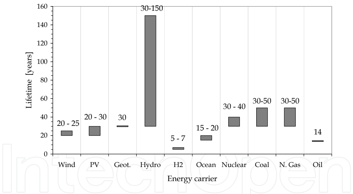
Fig. 3. Values range of lifetime (years) for each energy carrier.
