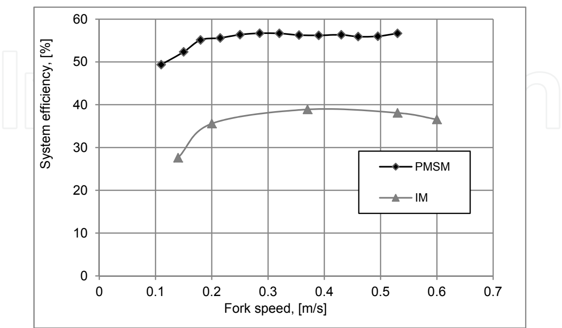
Fig. 10. System efficiency for lowering with 920 kg payload corresponding to 20 Nm shaft torque.
