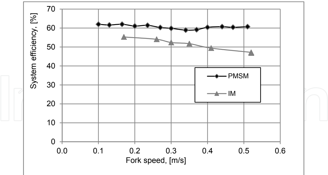
Fig. 9. System efficiency for lifting with 0 kg payload corresponding to 15 Nm shaft torque. In this case the PMSM brings clearly better results compared to the IM.
