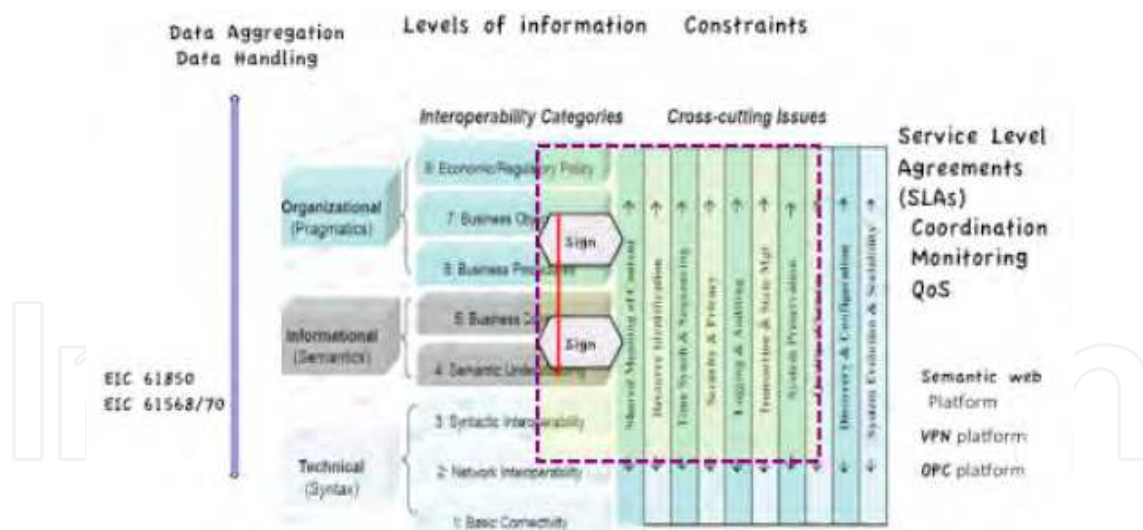
Fig. 11. The Interoperability Framework revisited. The vertical red line between signs illustrate verified interoperability.
