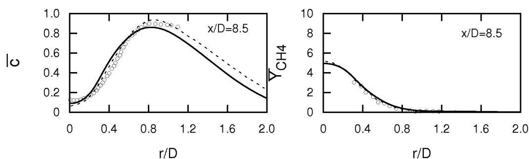
Fig. 6. The radial variation of \bar{c} and \bar{Y}_{CH_4} (in %) in flame F3; Fluent results (—), experimental measurements (○) and previously published results (---).
