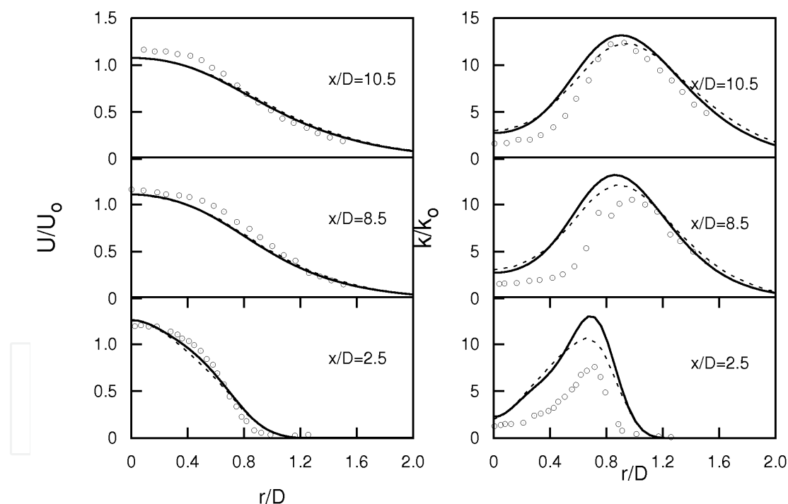
Fig. 4. The normalised mean axial velocity and turbulent kinetic energy in flame F1. Fluent ( — ) results are compared with experimental data ( \circ ) of Chen et al. (1996) and previously published results ( - - ) of Kolla & Swaminathan (2010b).
