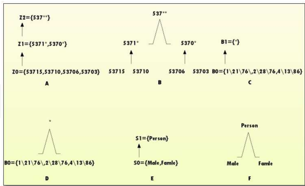
Fig. 6. Domain and value generalization hierarchies for Zip code (a, b), Birth Date (c, d), and Sex (e, f)(LeFevre, DeWitt et al. 2005).
