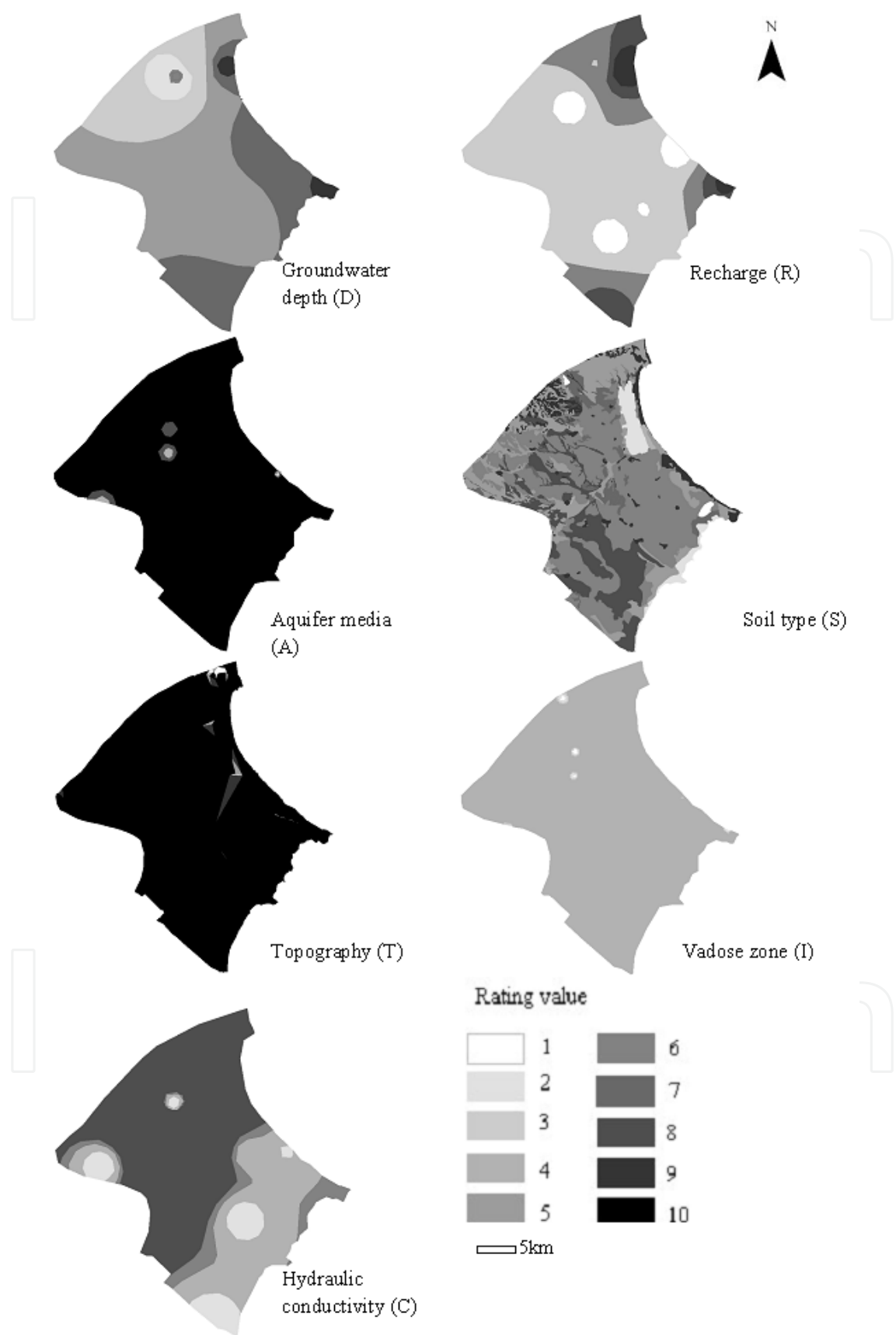
Fig. 2. Seven DRASTIC maps to compute the vulnerability index.
